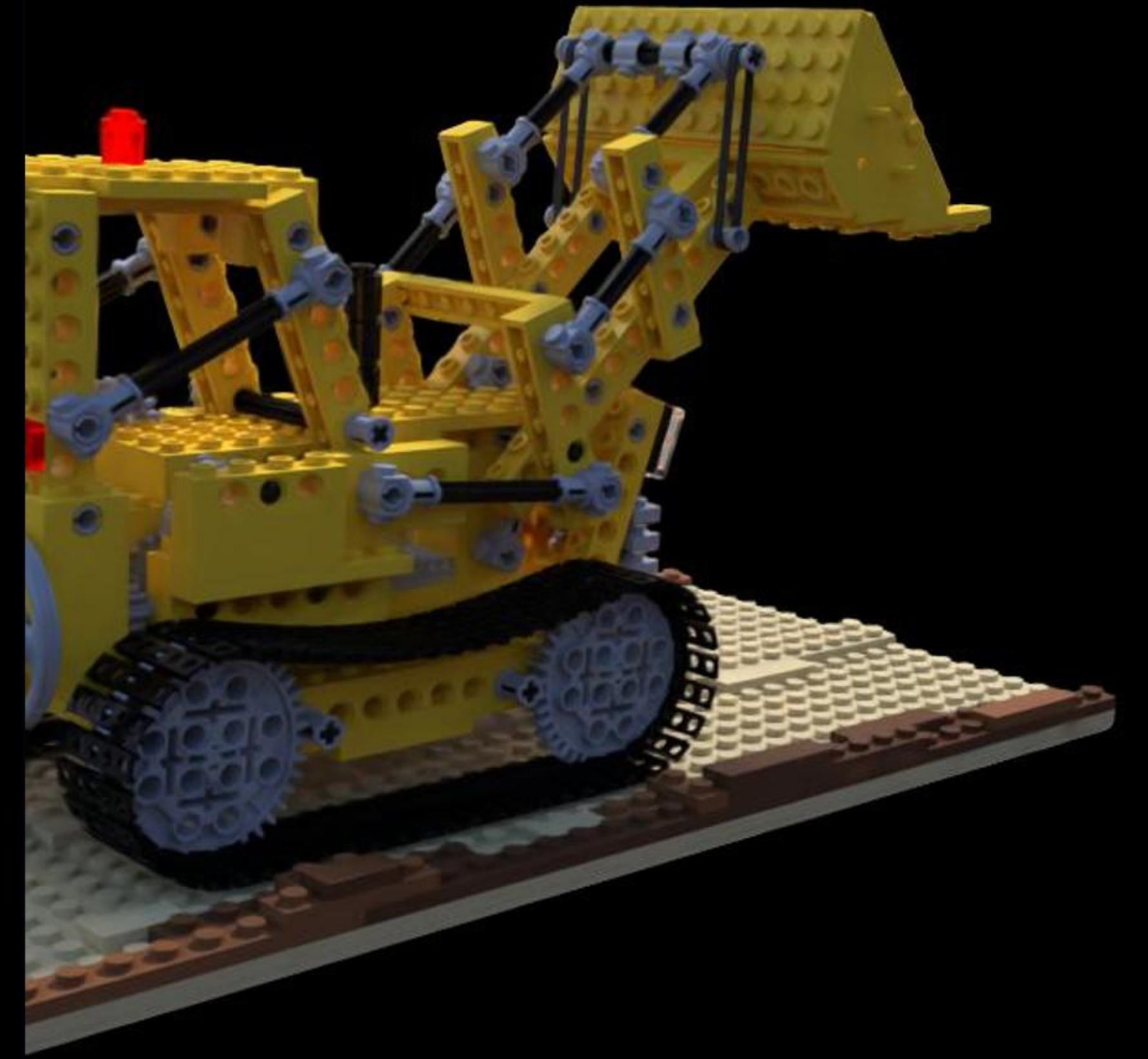
Config: COLMAP | | num_images=80 PSNR: 14.74 | LPIPS: 0.4265 | SSIM: 0.6160
