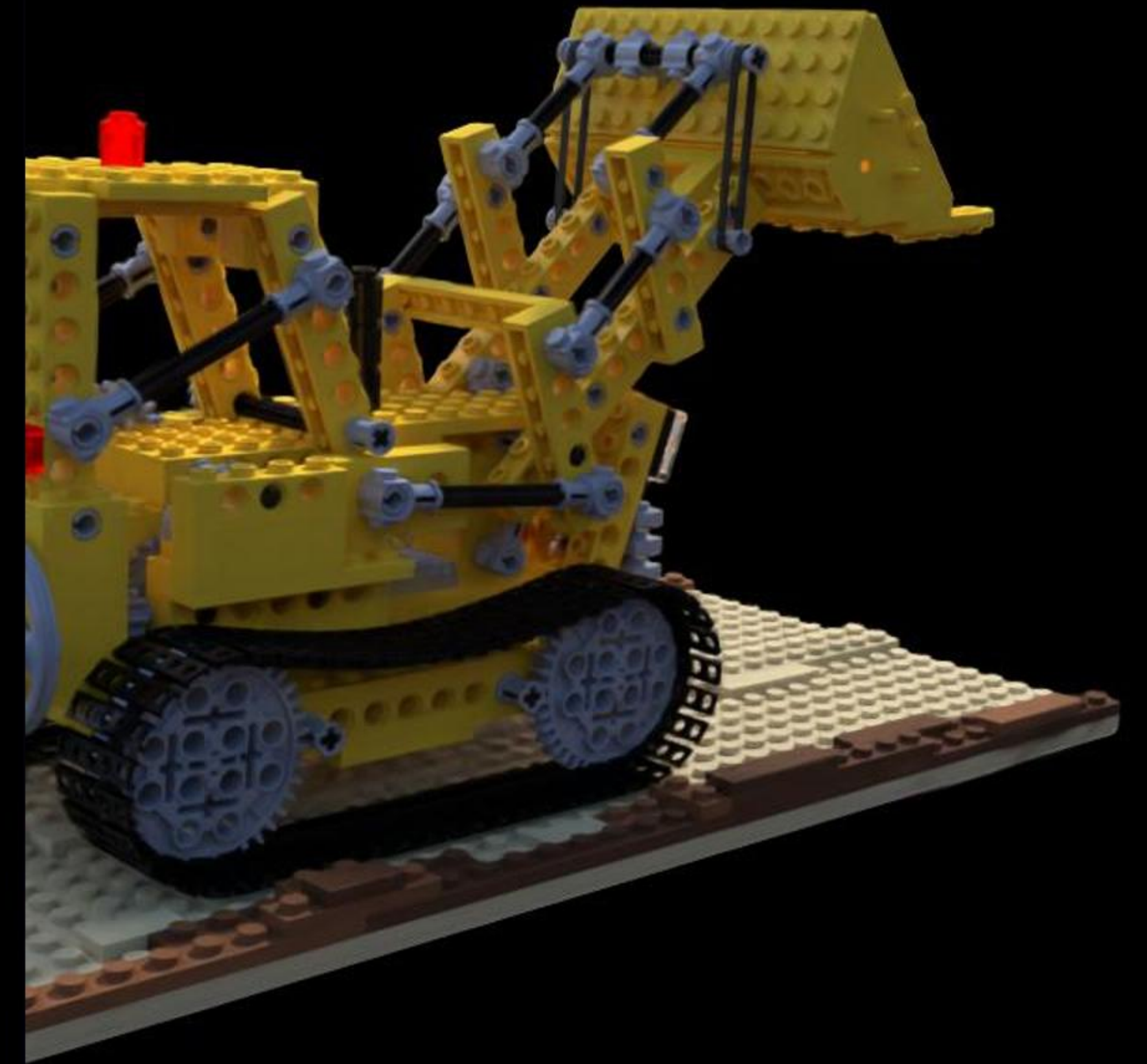
Config: COLMAP | | default PSNR: 14.73 | LPIPS: 0.4267 | SSIM: 0.6150
