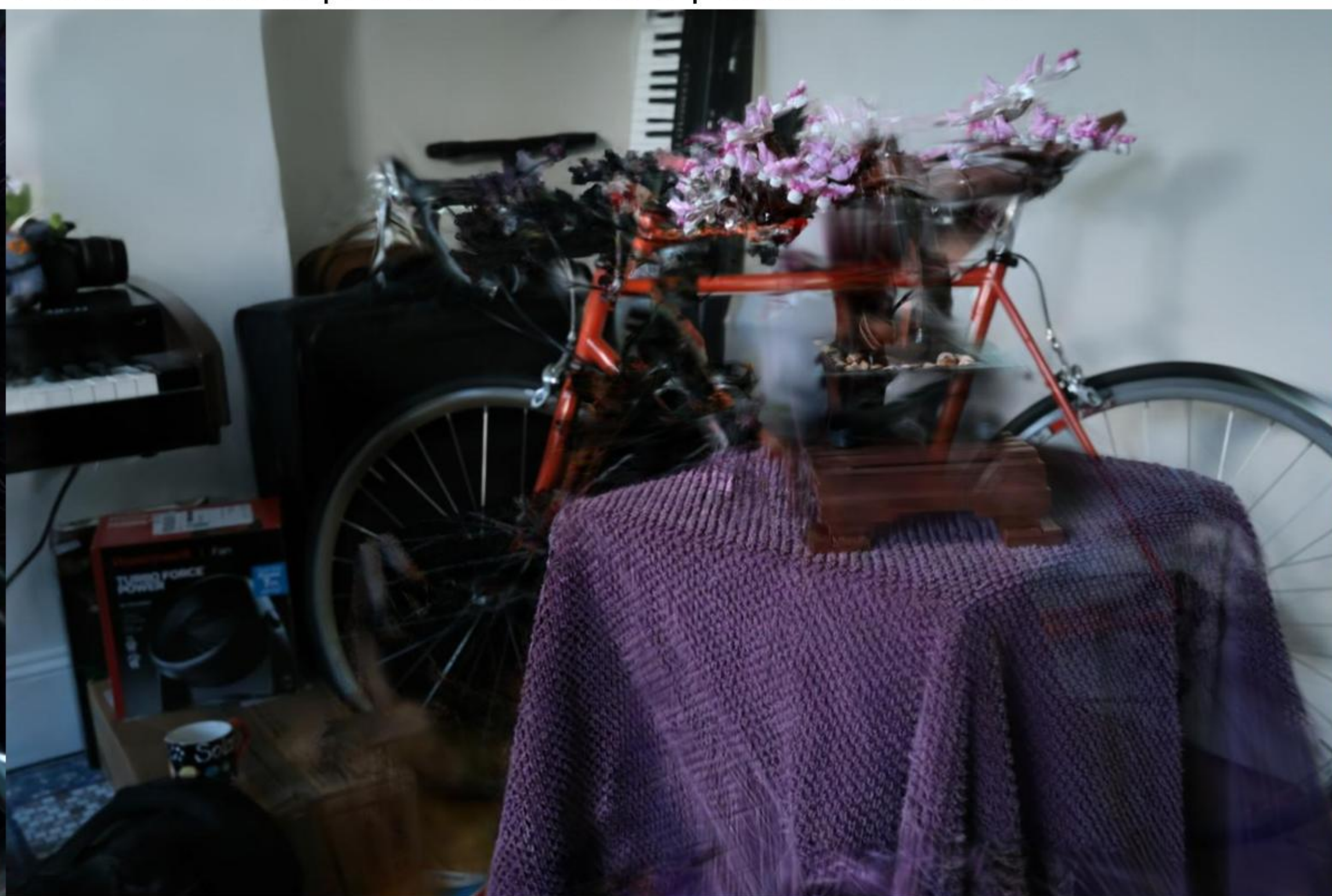
Config: COLMAP | farthestpose | num_images=40 PSNR: 13.28 | LPIPS: 0.5812 | SSIM: 0.4422
