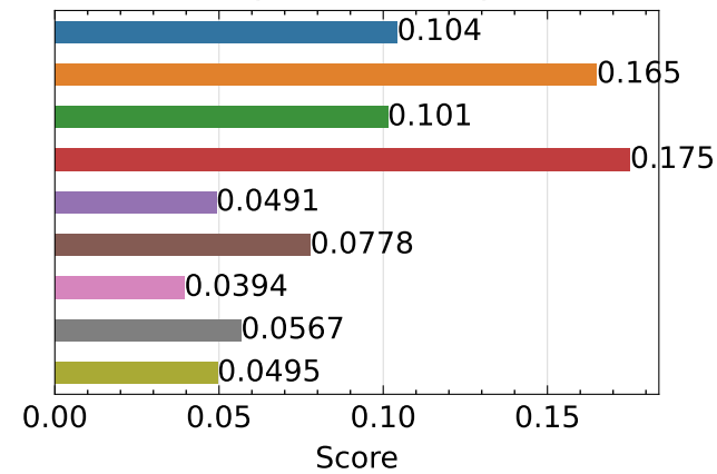
Composite Quality ↑
