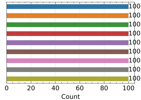
Composite Quality ↑
