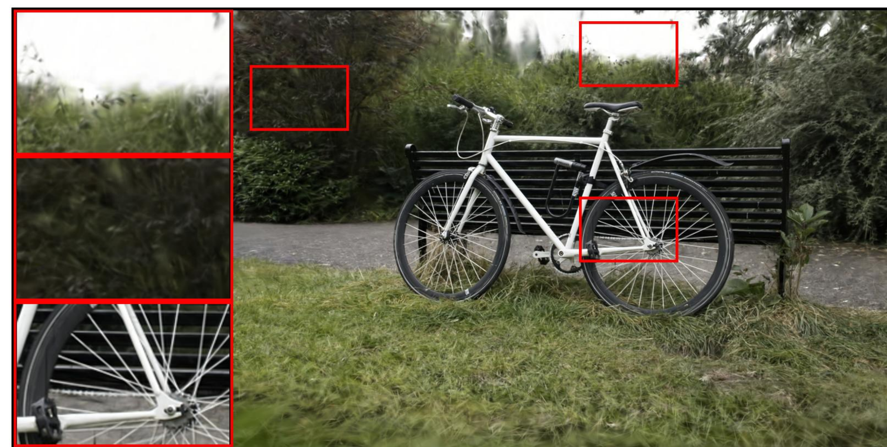
bicycle: VGGT | Pose Opt PSNR: 17.38 | LPIPS: 0.3378 | SSIM: 0.2679
