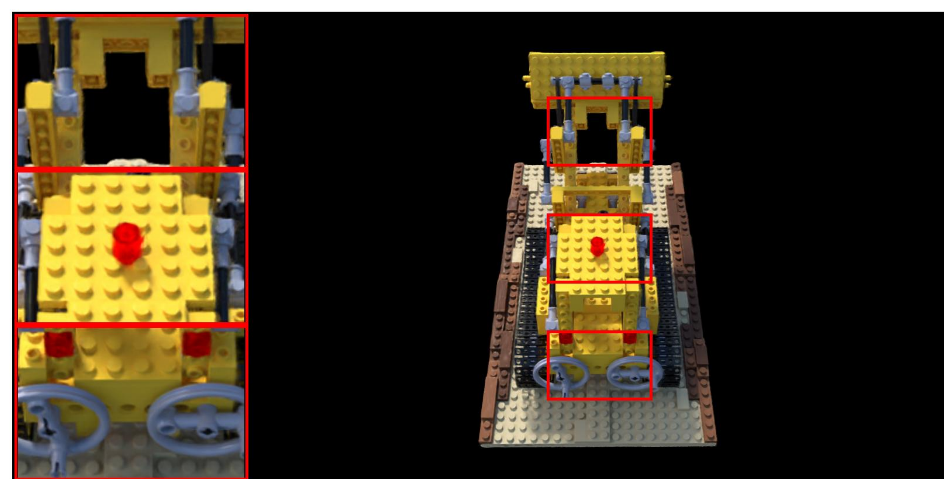
lego: VGGT | PSNR: 20.57 | LPIPS: 0.0950 | SSIM: 0.7737
