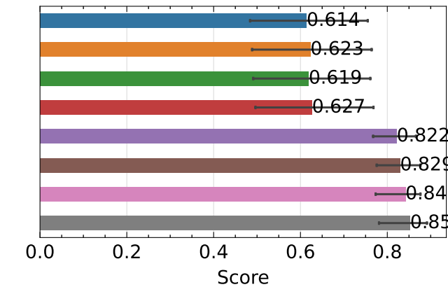
Composite Quality ↑ - colmap - indoor
