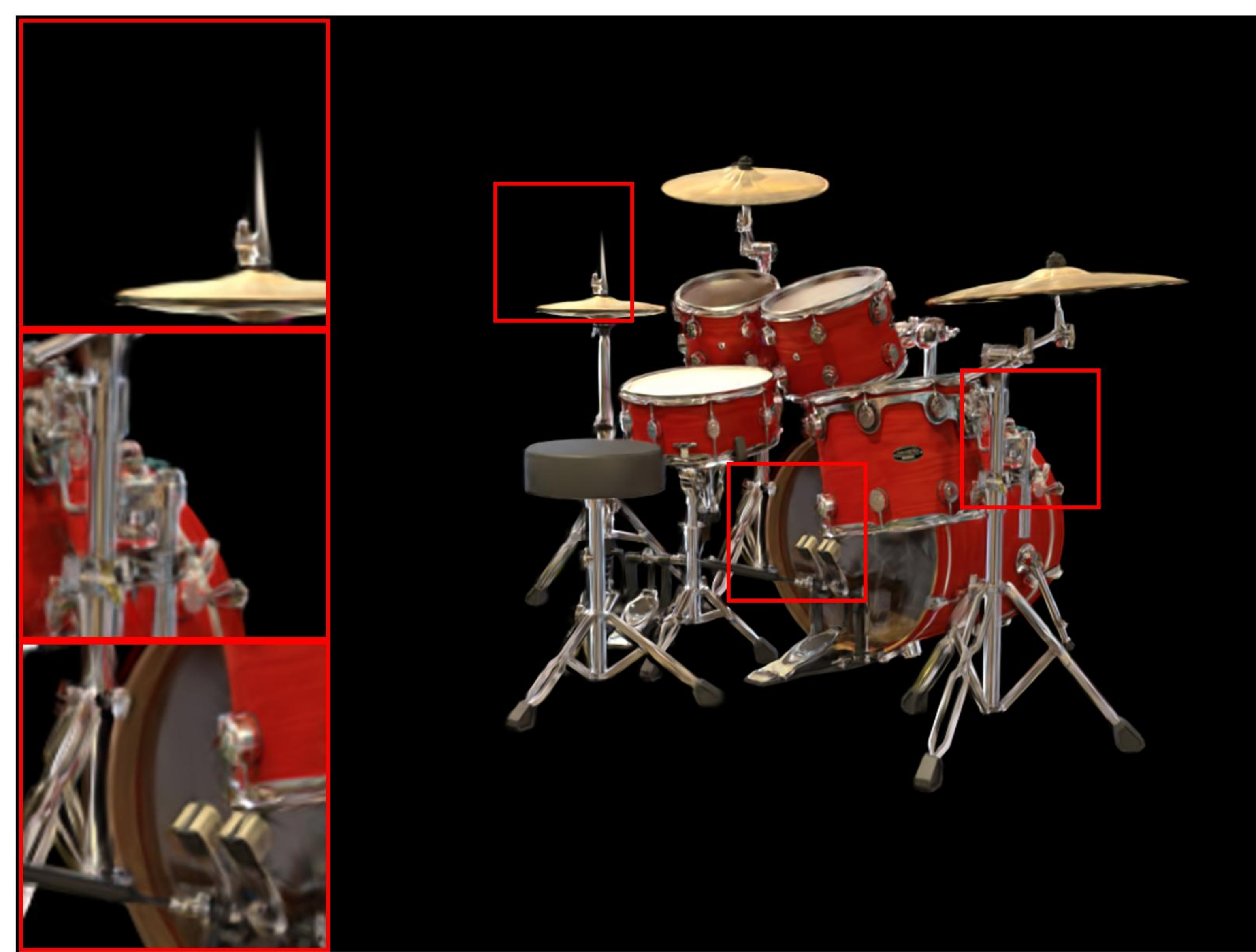
drums: VGGT | Random Init | Use BA | real_num_points=3866 PSNR: 18.61 | LPIPS: 0.1225 | SSIM: 0.8162
