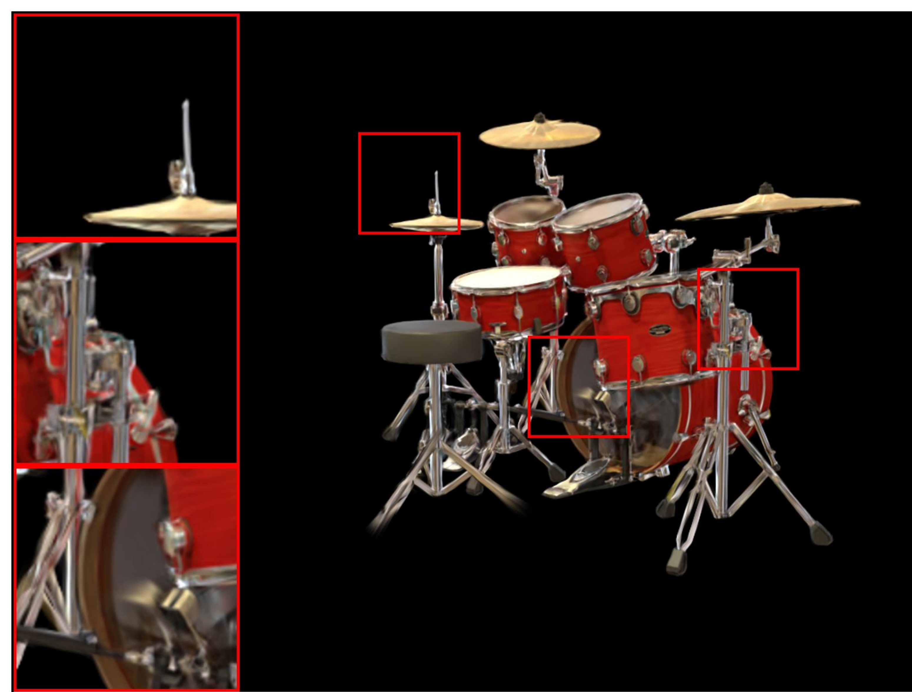
drums: VGGT | Random Init | | real_num_points=3866 PSNR: 19.70 | LPIPS: 0.1263 | SSIM: 0.8378
