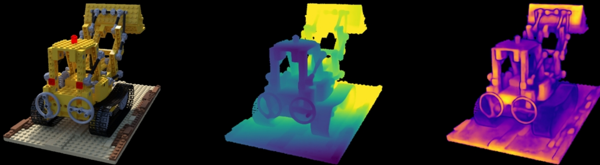
lego: VGGT | | Original | Depth (max=1.28) | Confidence (max=155.74)
