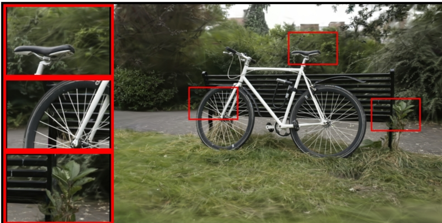
bicycle: COLMAP | | | num_points=17352 PSNR: 22.16 | LPIPS: 0.3495 | SSIM: 0.5587
