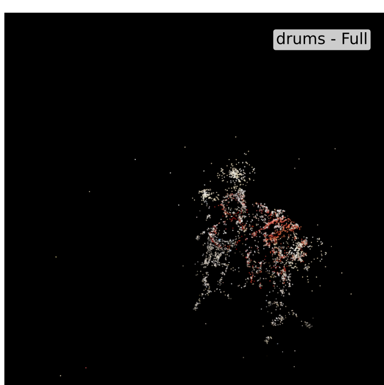
COLMAP | | |
