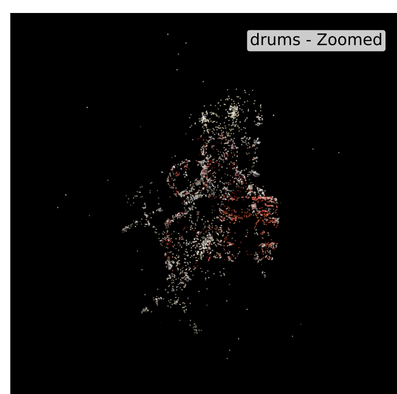
COLMAP | | |
