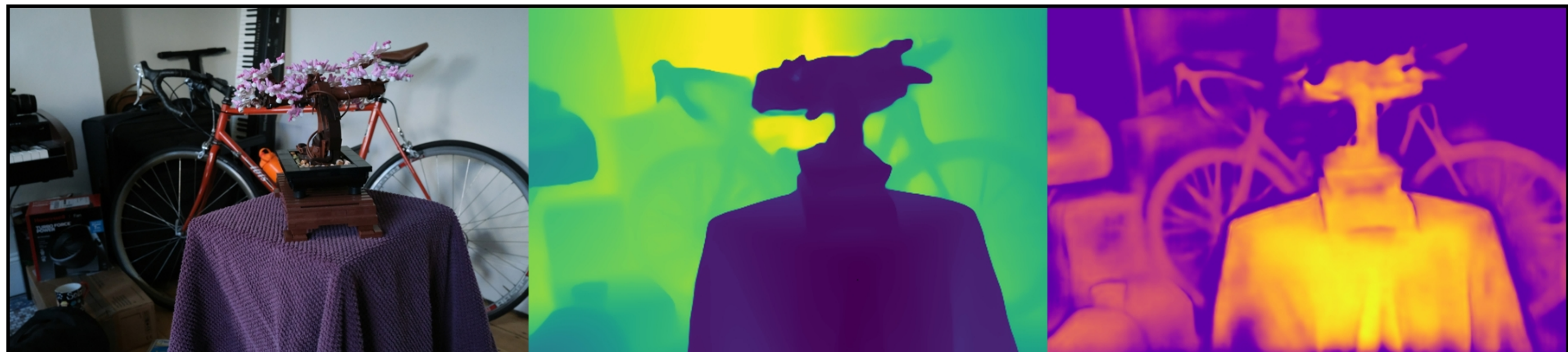
bonsai: Combined | COLMAP Cams | VGGT Pcd | confidence Original | Depth (max=15.46) | Confidence (max=35.95)
