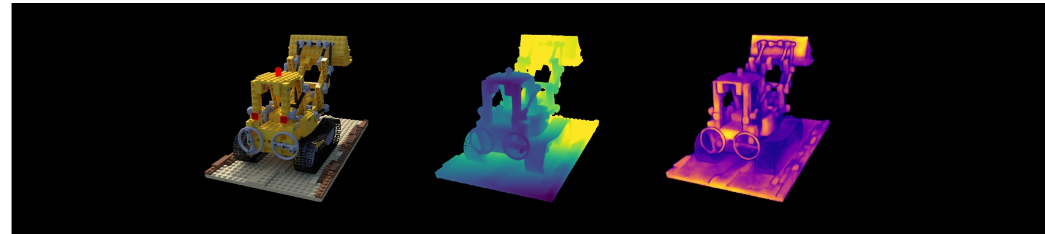
lego: Combined | COLMAP Cams | VGGT Pcd | confidence Original | Depth (max=5.88) | Confidence (max=713.75)
