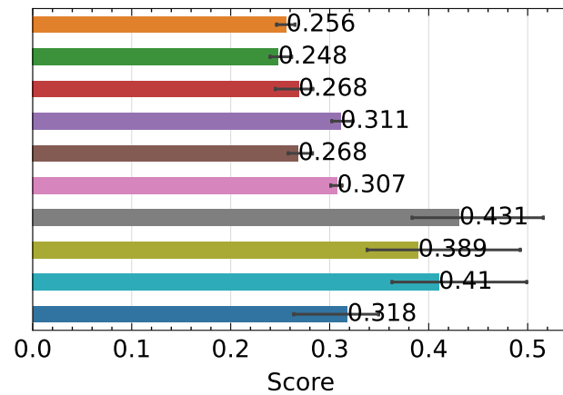
SSIM ↑ - outdoor
