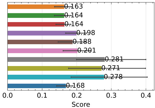
SSIM ↑ - indoor
