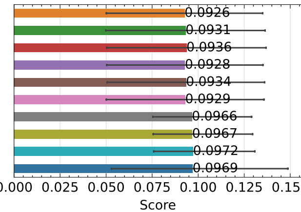
SSIM ↑ - synthetic
