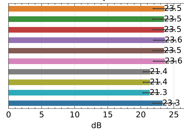
PSNR ↑ - synthetic
