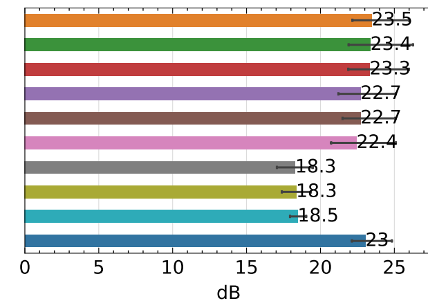
PSNR ↑ - outdoor
