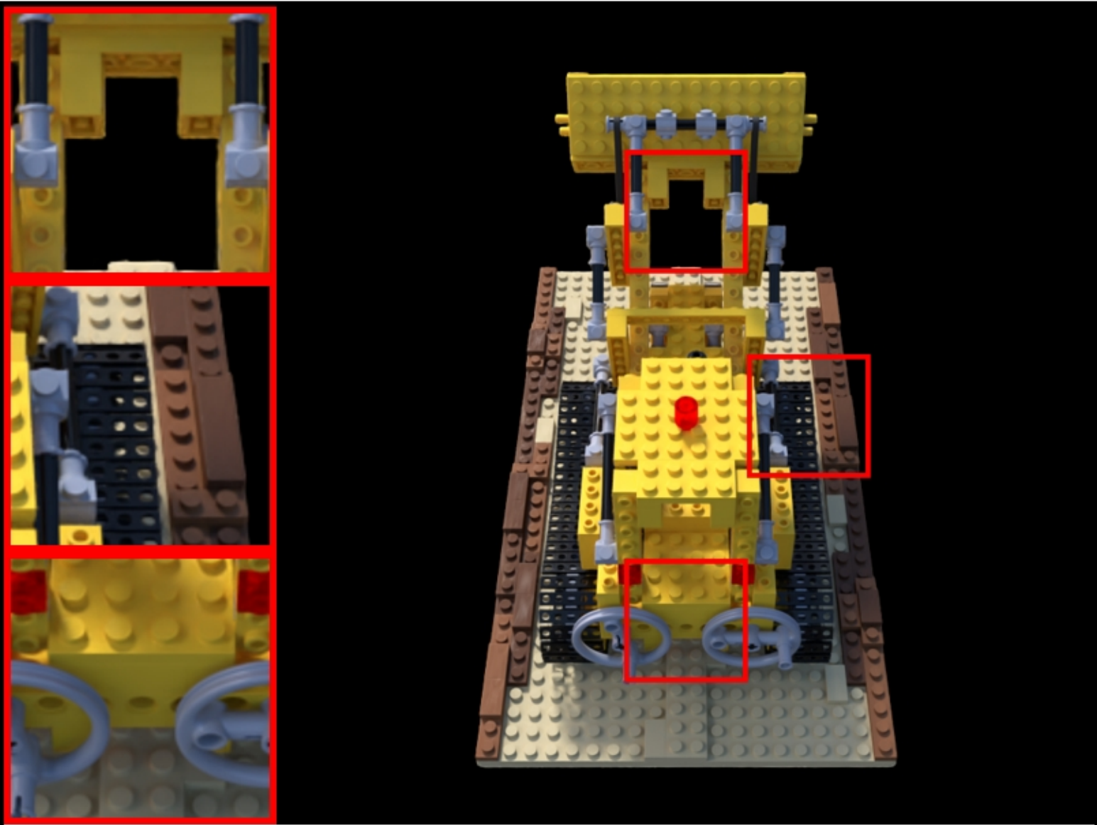
lego: Combined | COLMAP Cams | VGGT Pcd | confidence PSNR: 25.25 | LPIPS: 0.0504 | SSIM: 0.9047
