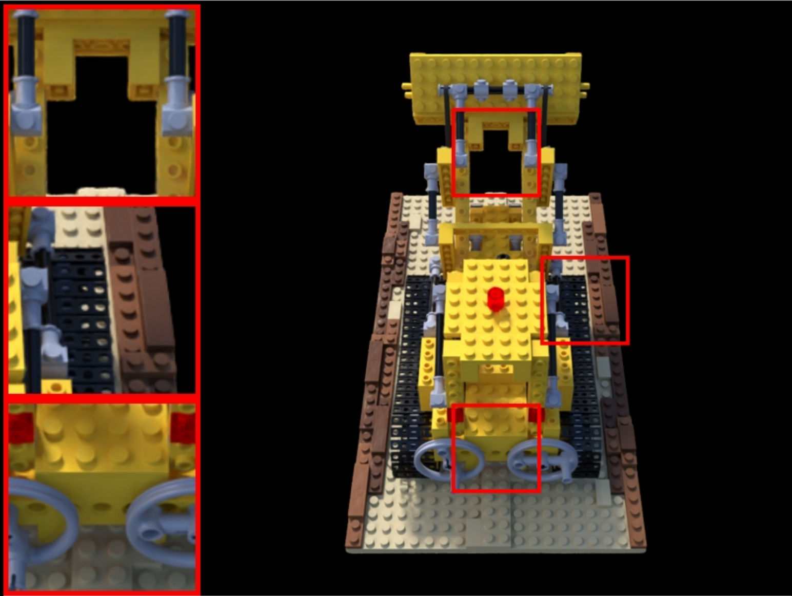
lego: VGGT | | random PSNR: 20.38 | LPIPS: 0.0756 | SSIM: 0.7739
