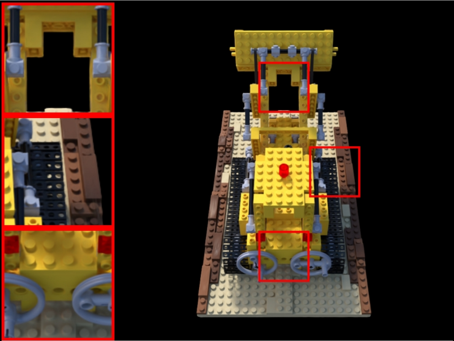
lego: COLMAP | | confidence PSNR: 25.24 | LPIPS: 0.0529 | SSIM: 0.9057
