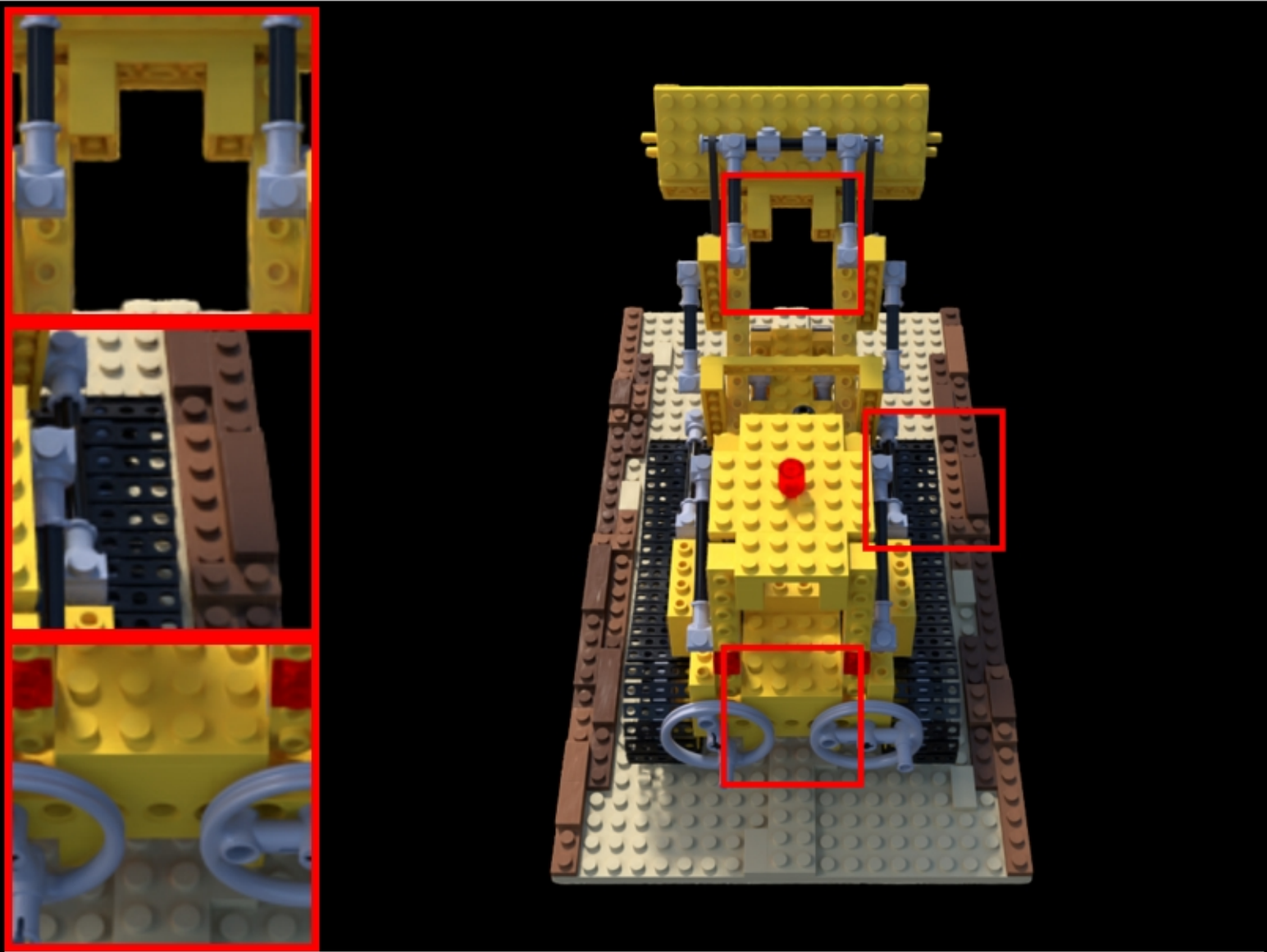
lego: VGGT | | confidence PSNR: 20.37 | LPIPS: 0.0754 | SSIM: 0.7739
