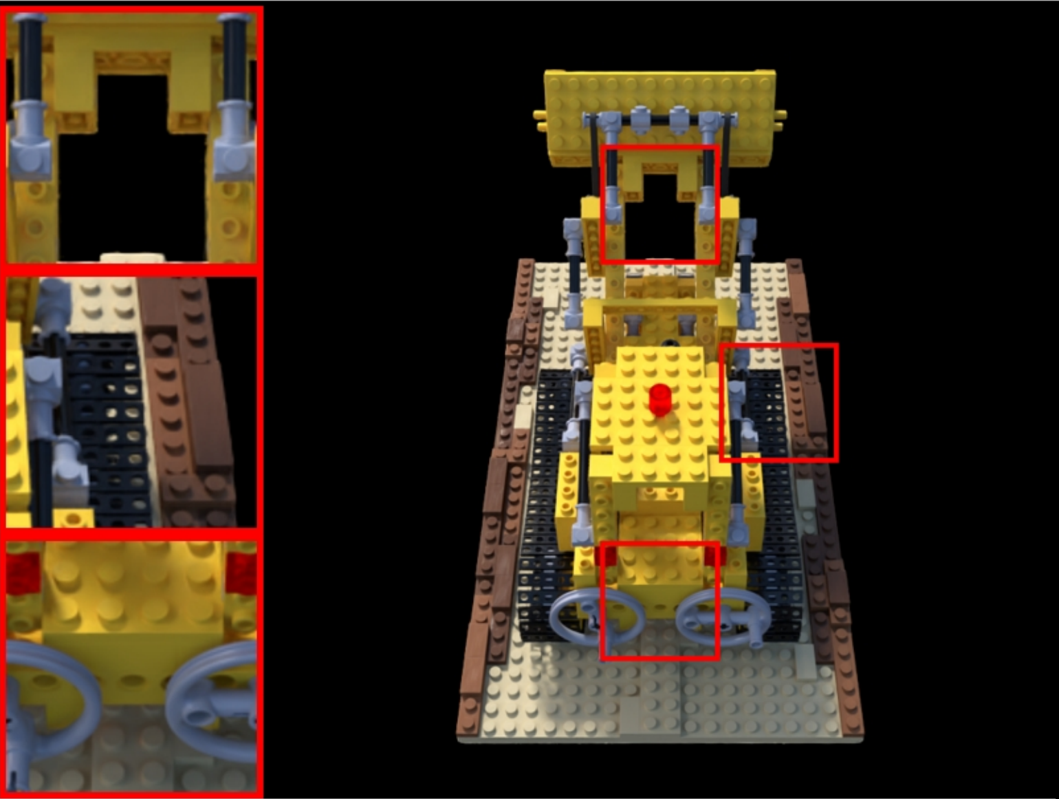
lego: Combined | COLMAP Cams | VGGT Pcd | voxels PSNR: 25.32 | LPIPS: 0.0501 | SSIM: 0.9053
