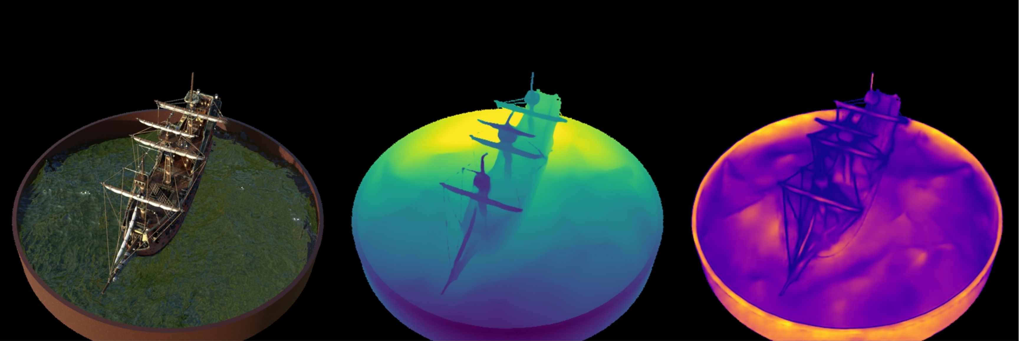
ship: Combined | COLMAP Cams | Both Pcds | voxels Original | Depth (max=6.66) | Confidence (max=793.41)
