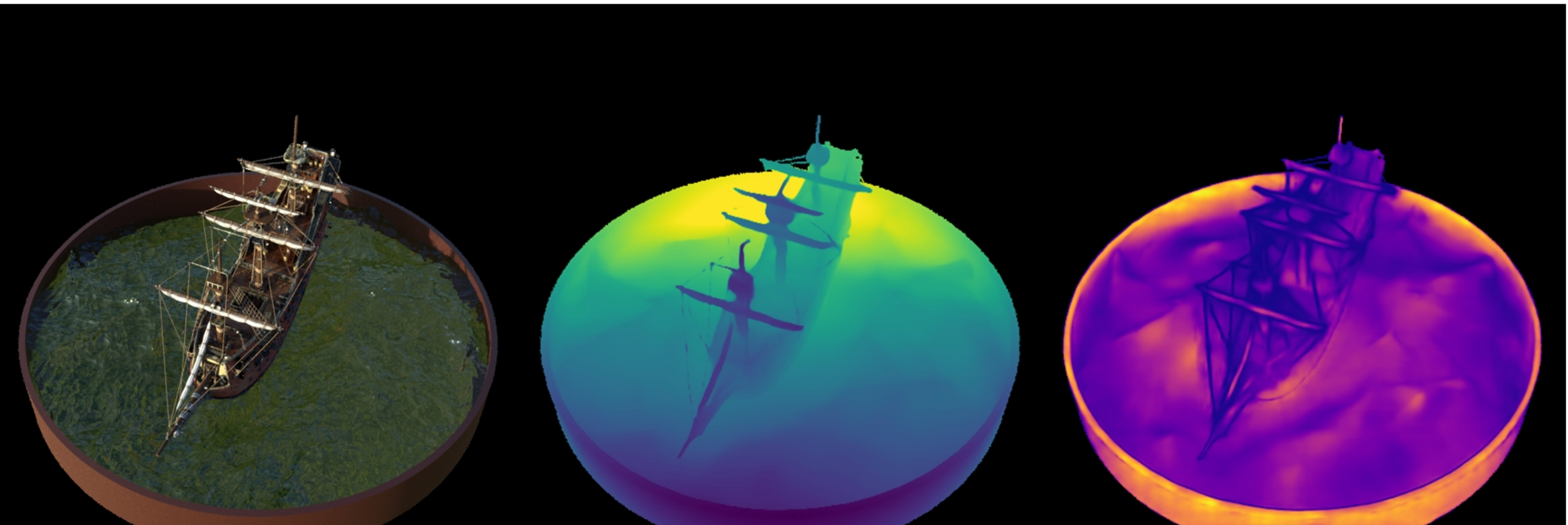
ship: Combined | COLMAP Cams | VGGT Pcd | voxels Original | Depth (max=6.66) | Confidence (max=793.41)
