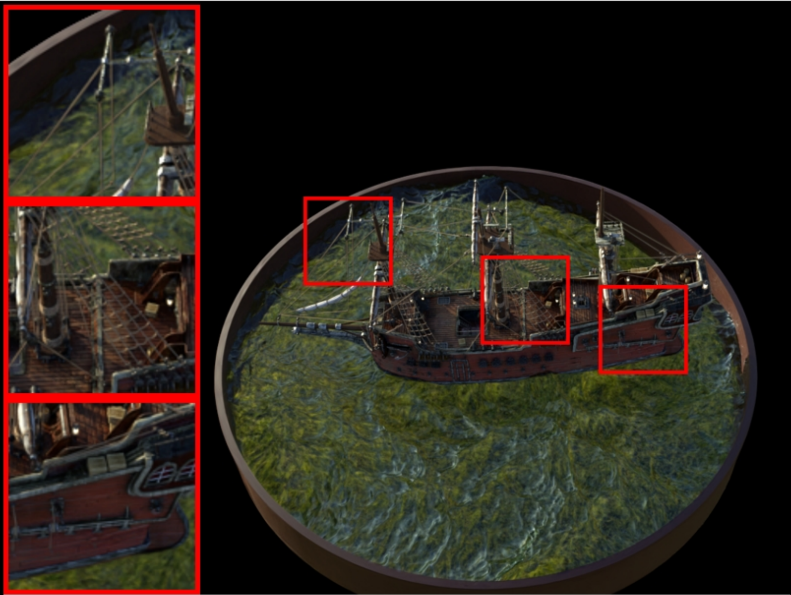
ship: Combined | COLMAP Cams | VGGT Pcd | random PSNR: 21.83 | LPIPS: 0.1361 | SSIM: 0.7338
