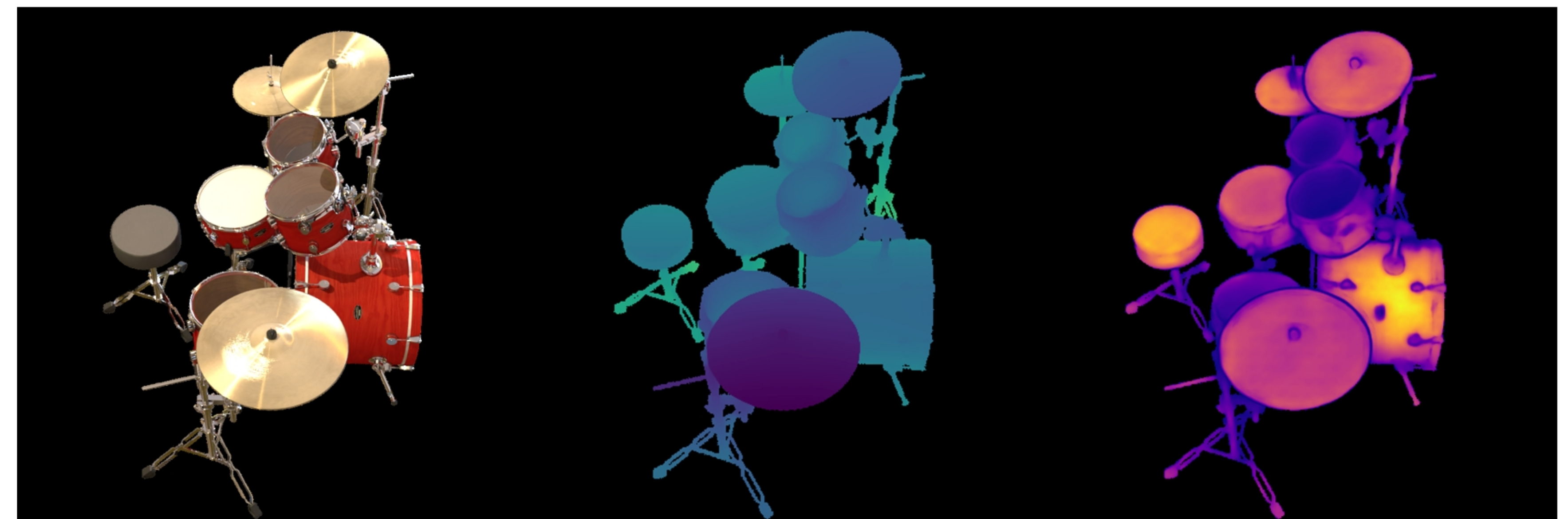
drums: VGGT | | num_images=70
