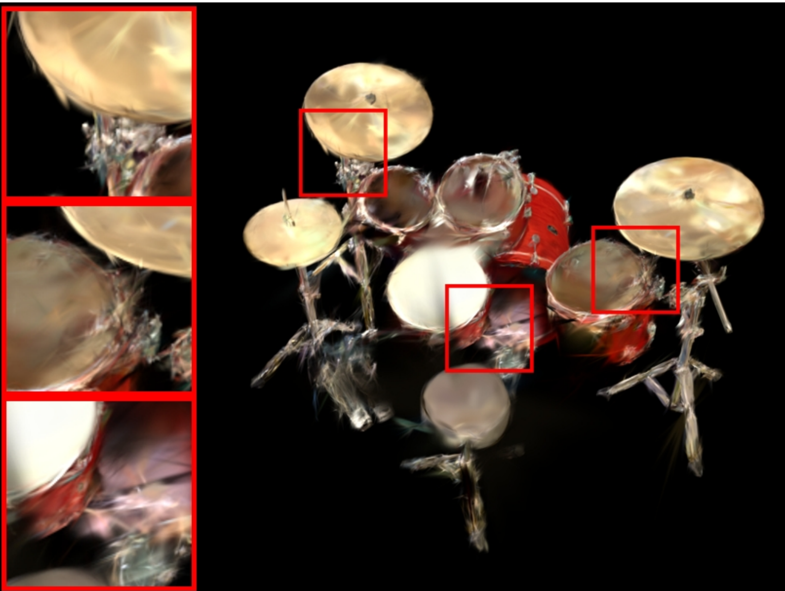
drums: COLMAP | num_images=70 PSNR: 16.65 | LPIPS: 0.1717 | SSIM: 0.7655
