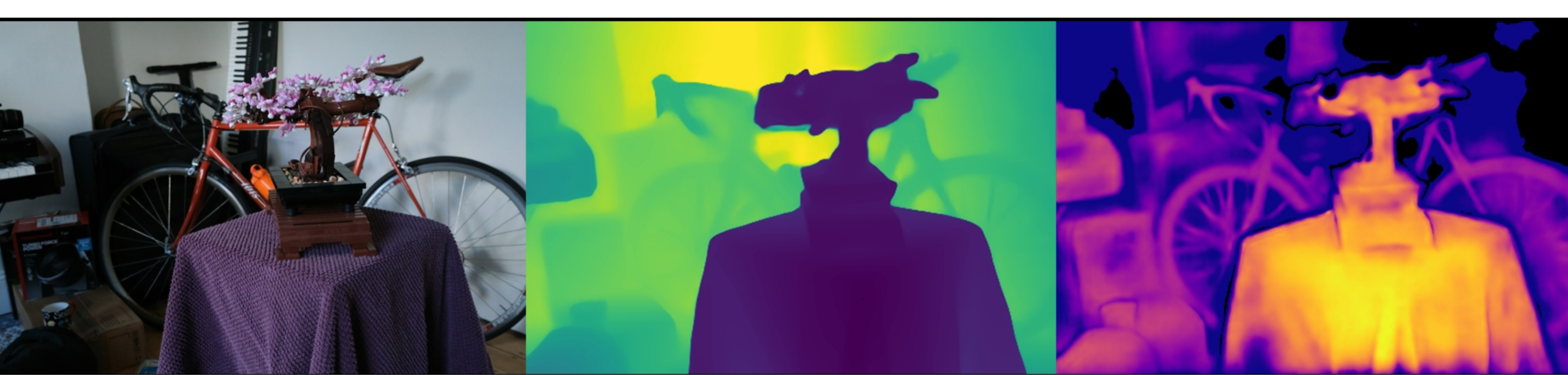
bonsai: VGGT | 1.0 Original | Depth (max=2.21) | Confidence (max=5.14)
