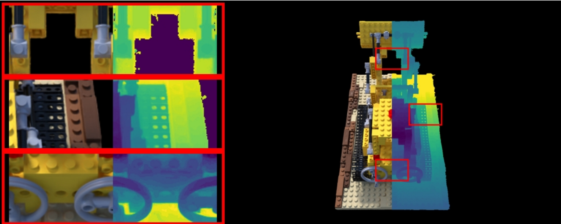
lego: VGGT | 10.0 PSNR: 20.34 | LPIPS: 0.0759 | SSIM: 0.7733
