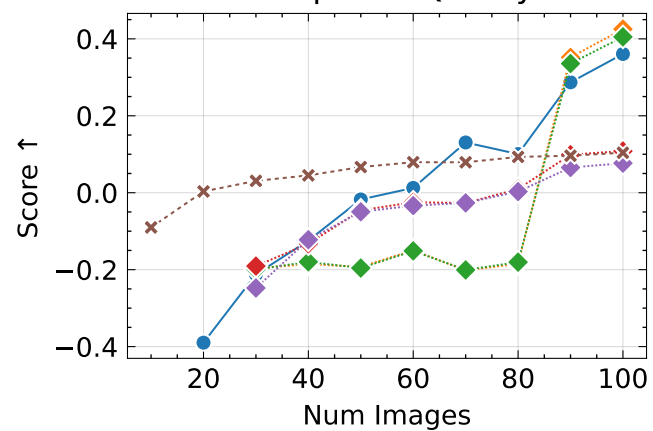
Composite Quality
