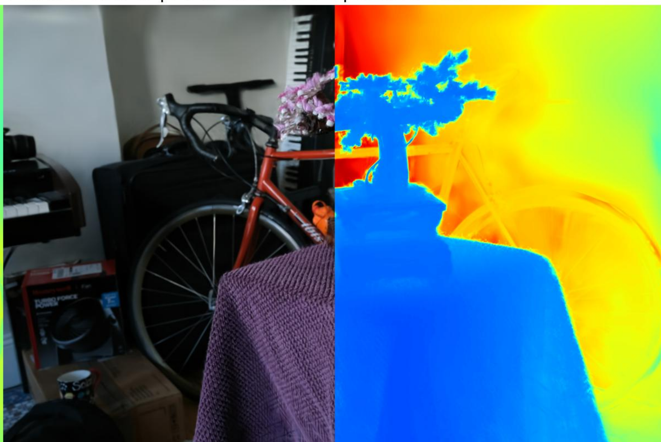
Config: VGGT | standard | depth_lambda=0.01 PSNR: 17.28 | LPIPS: 0.3296 | SSIM: 0.5687
