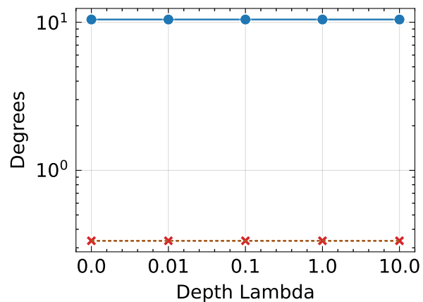
RRE ↓
