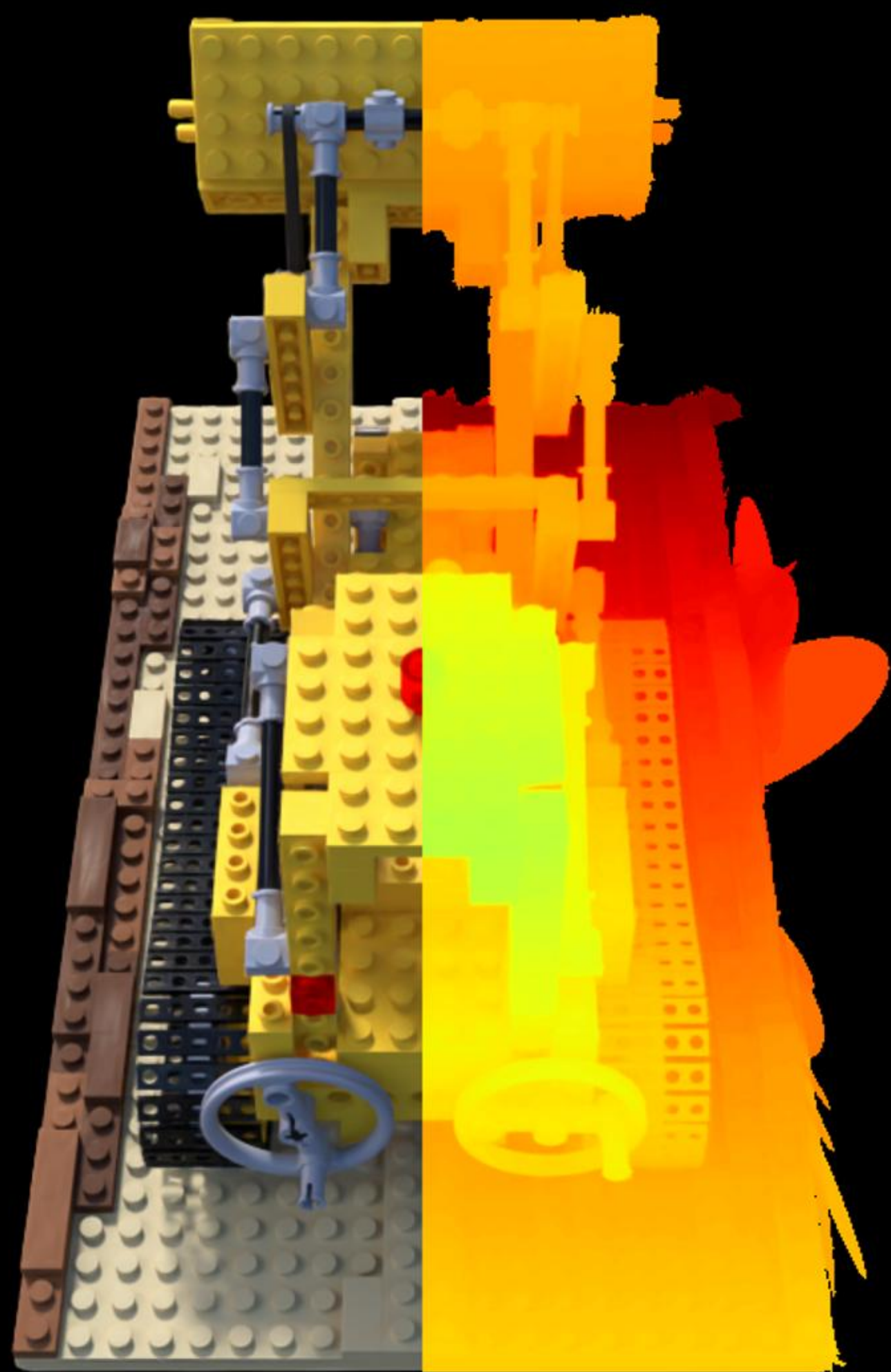
Config: COLMAP | | depth_lambda=0.01 PSNR: 25.12 | LPIPS: 0.0522 | SSIM: 0.9102
