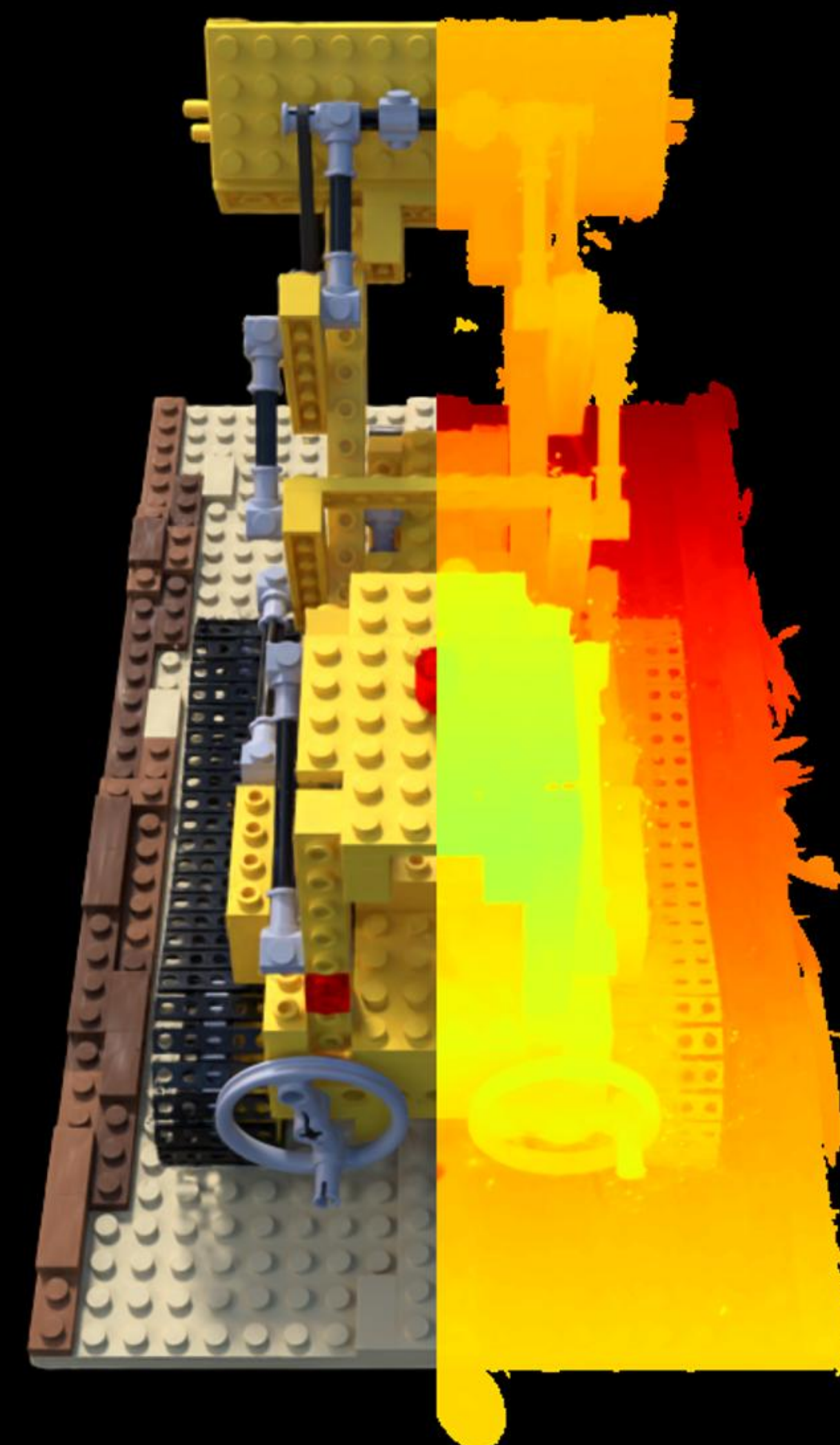
Config: COLMAP | | depth_lambda=1.0 PSNR: 25.34 | LPIPS: 0.0530 | SSIM: 0.9119
