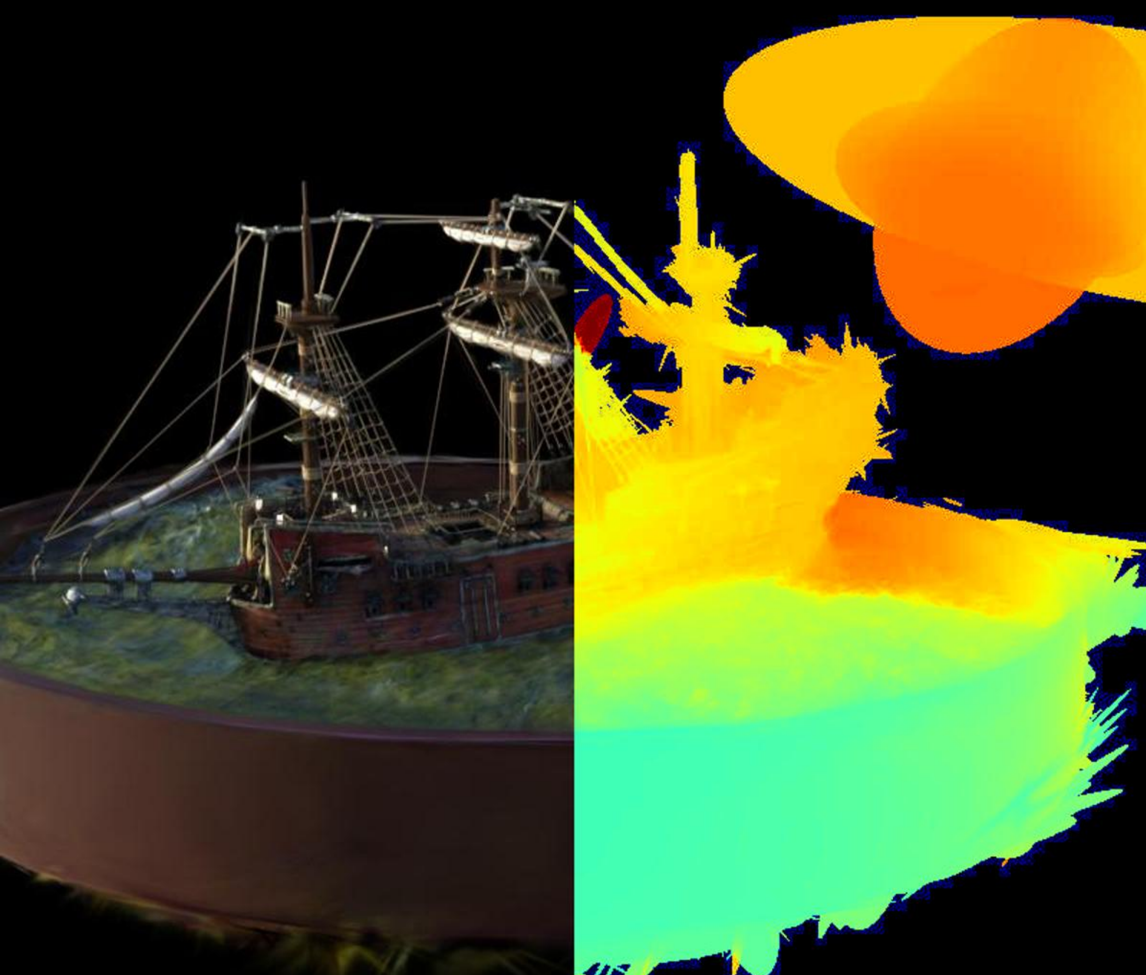
Config: COLMAP | | depth_lambda=0.0 PSNR: 22.21 | LPIPS: 0.1732 | SSIM: 0.6646
