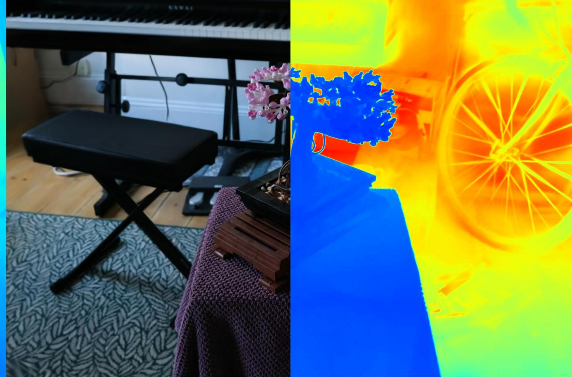
Config: COLMAP | PSNR: 24.99 | LPIPS: 0.1108 | SSIM: 0.7608
