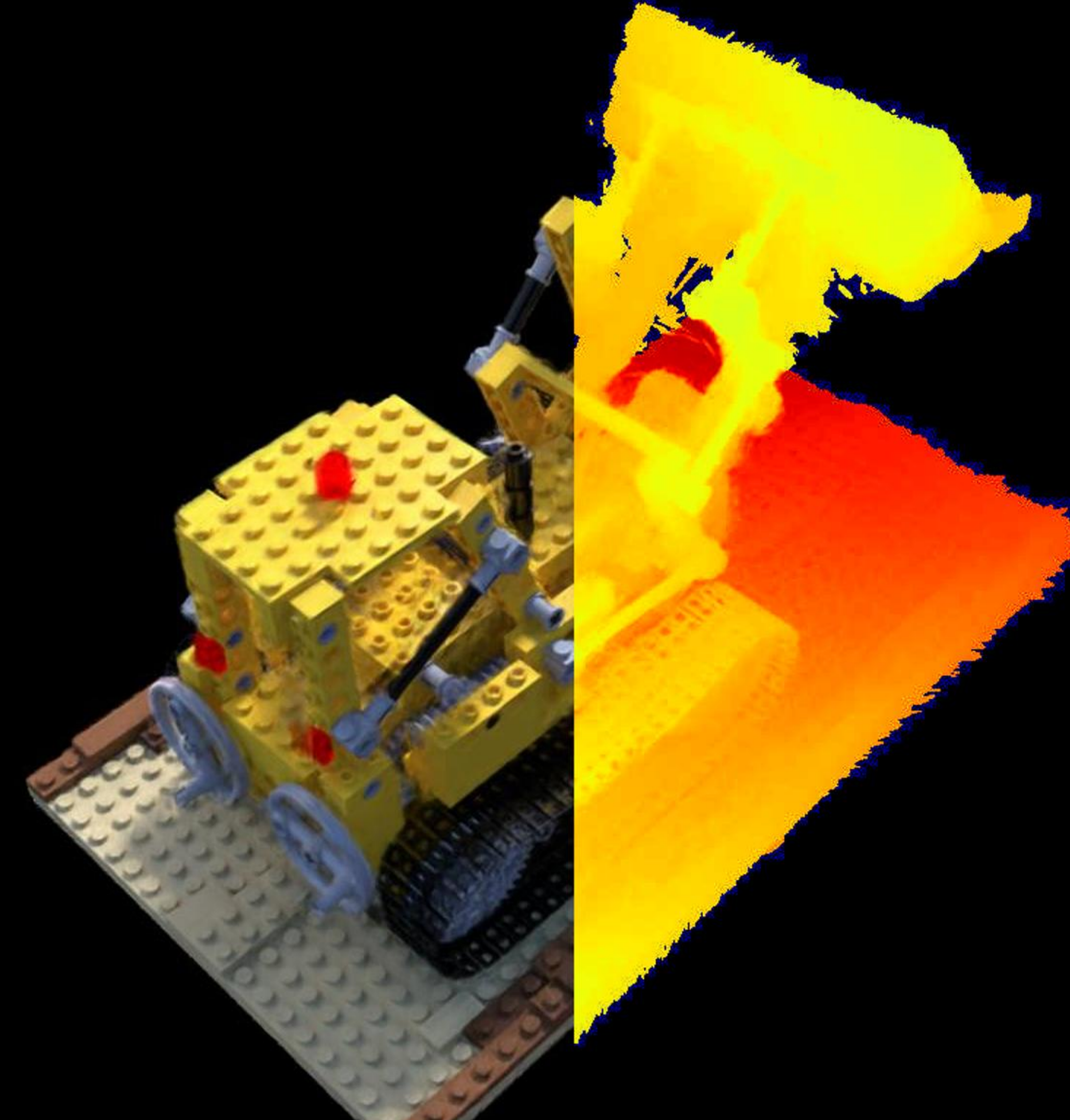
Config: VGGT | standard PSNR: 14.99 | LPIPS: 0.2798 | SSIM: 0.6312
