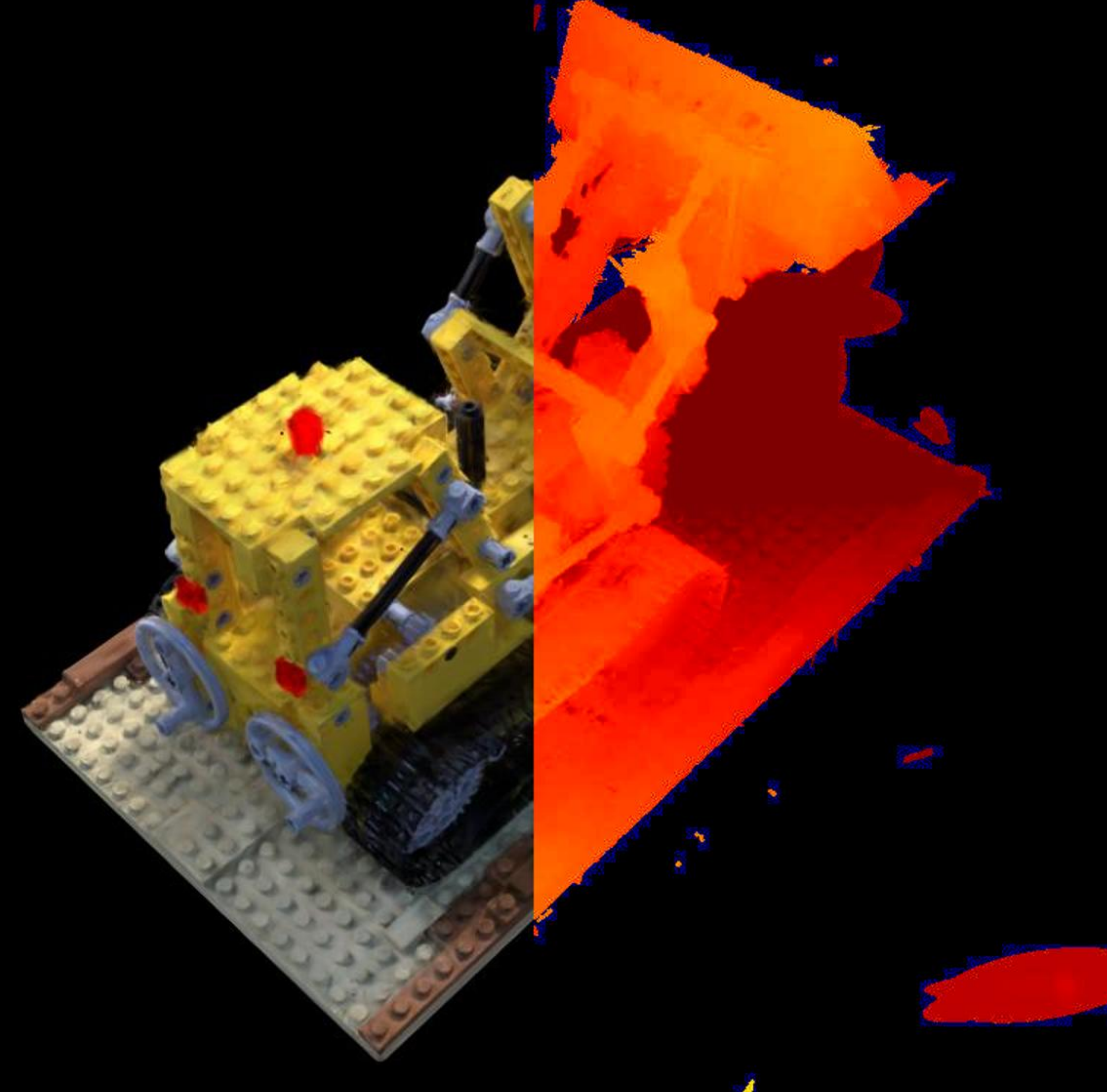
Config: COLMAP | PSNR: 22.41 | LPIPS: 0.0892 | SSIM: 0.8533
