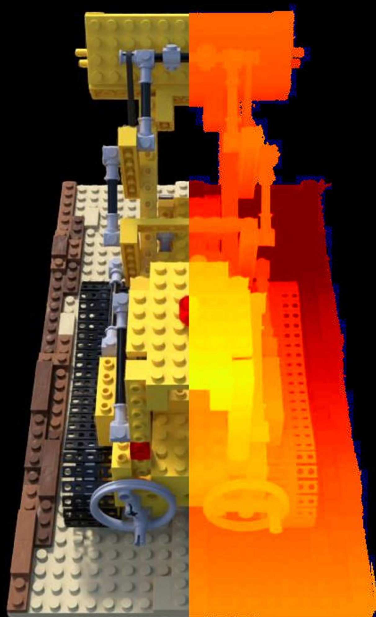
Config: VGGT | standard | depth_lambda=0.0 PSNR: 26.03 | LPIPS: 0.0447 | SSIM: 0.9341
