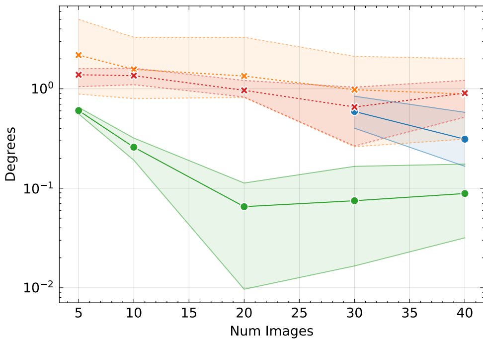
Aligned Cameras ↑
