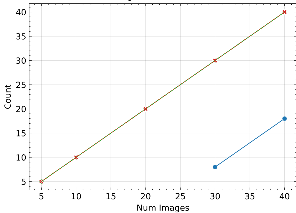
Aligned Cameras ↑
