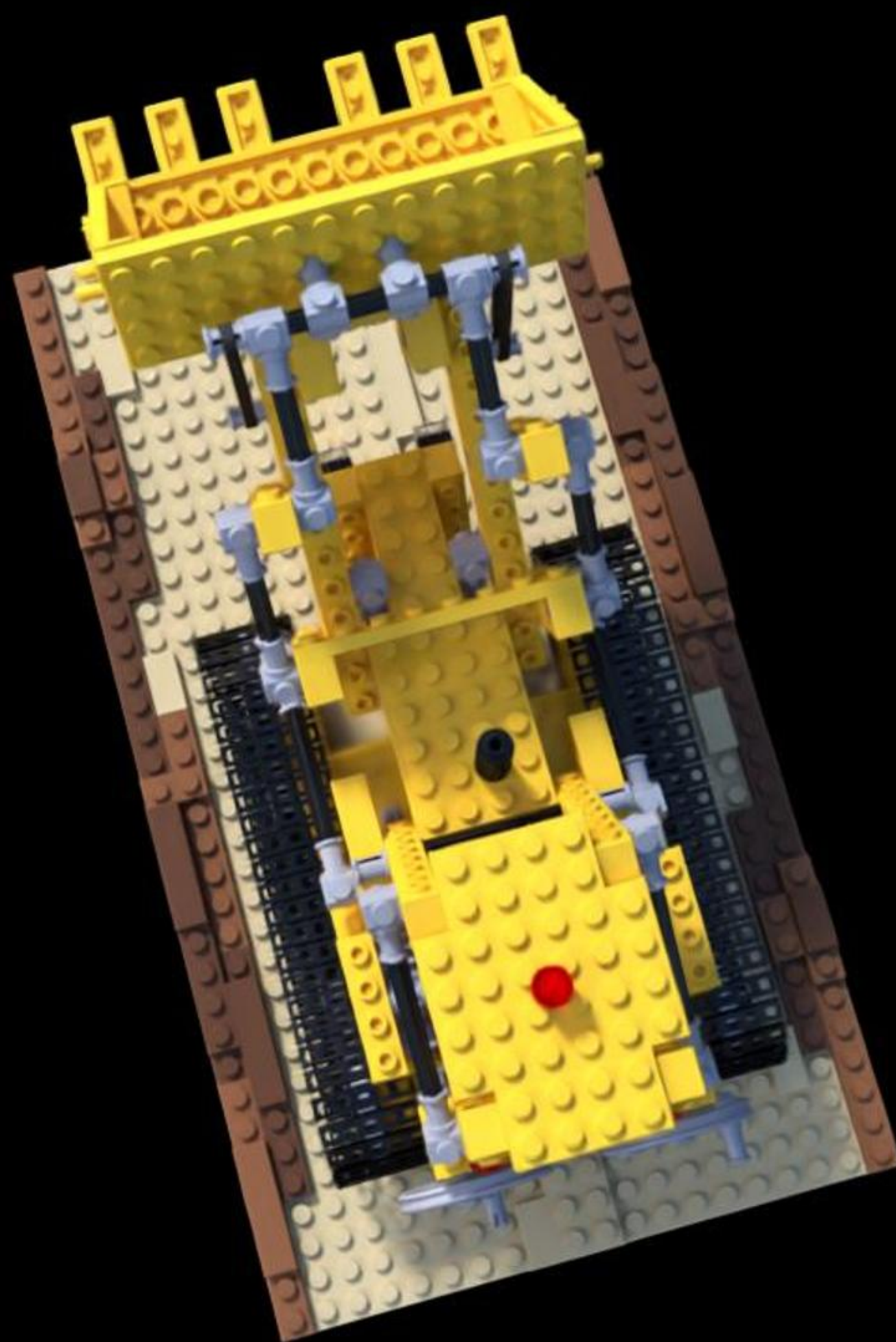
Config: VGGT | mcmc | Pose Opt | val_step=15000 PSNR: 20.87 | LPIPS: 0.0731 | SSIM: 0.7932
