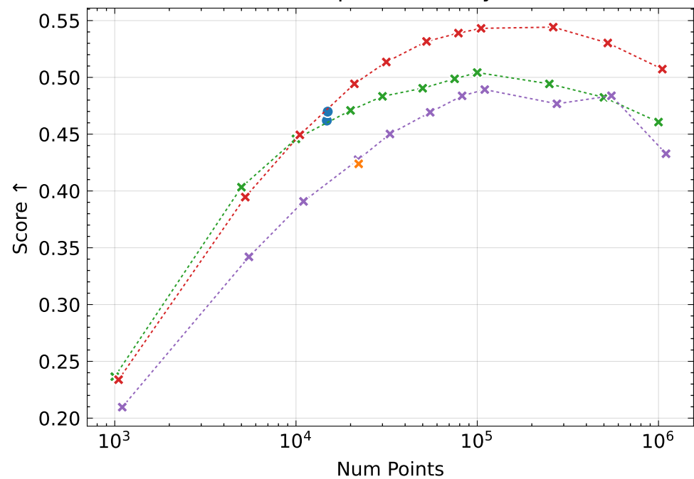
Composite Quality
