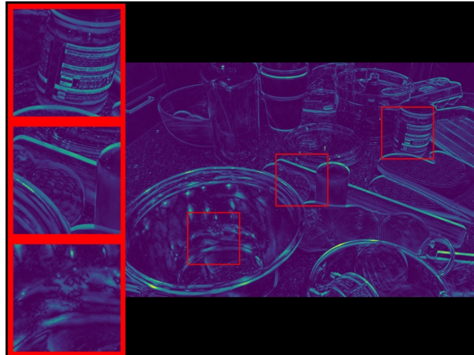
counter: VGGT | num_images=100 PSNR: 20.05 | LPIPS: 0.2915 | SSIM: 0.6178
