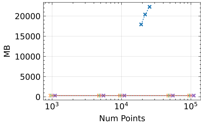
Pcd Processing Peak Memory ↓ - indoor
