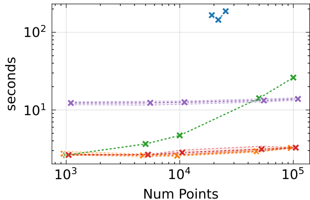
Pcd Processing Time ↓ - indoor
