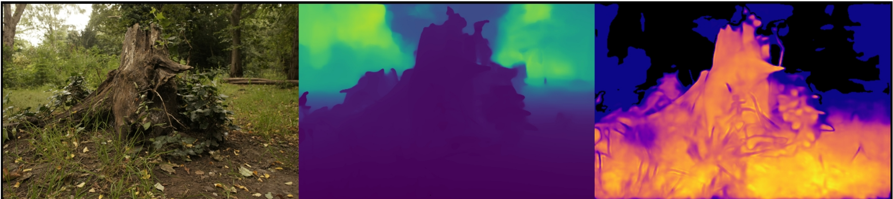
stump: VGGT | ba | num_points=21431 Original | Depth (max=6.21) | Confidence (max=3.47)
