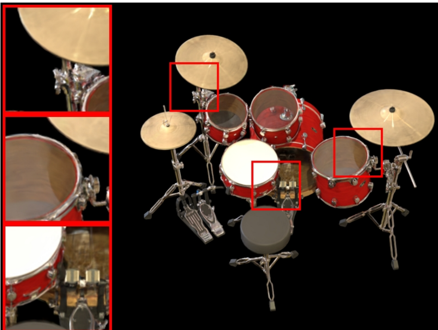
drums: VGGT | ba | num_points=26382 PSNR: 18.58 | LPIPS: 0.1111 | SSIM: 0.8146
