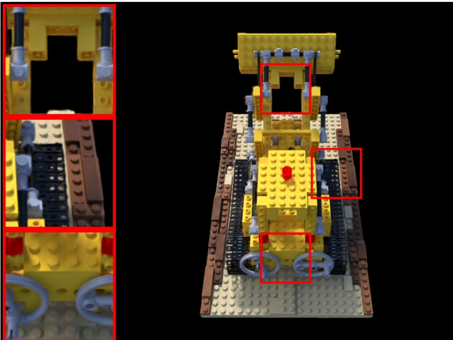
lego: VGGT | ba | num_points=27774 PSNR: 22.97 | LPIPS: 0.0746 | SSIM: 0.8368
