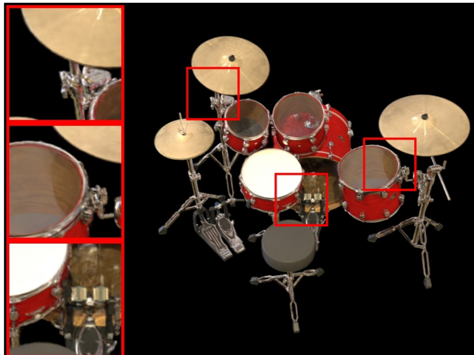
drums: VGGT | random | num_points=87000 PSNR: 19.68 | LPIPS: 0.1062 | SSIM: 0.8359
