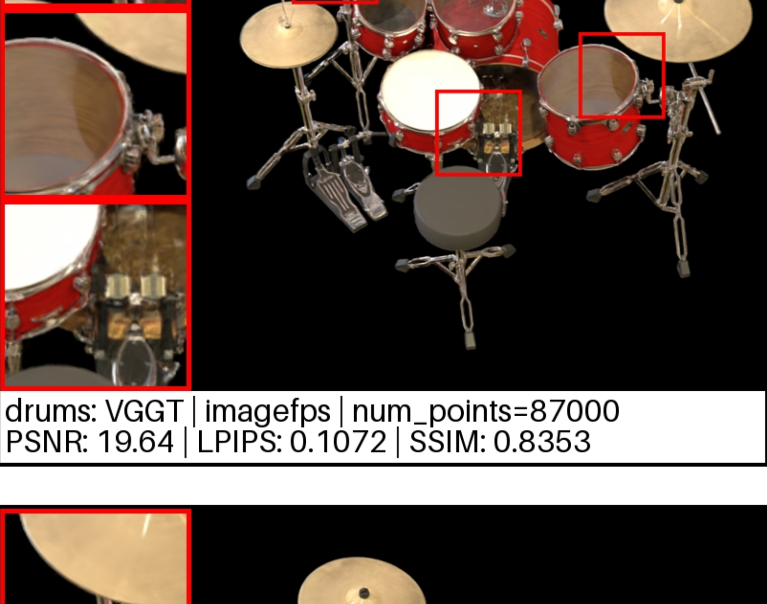
drums: VGGT | imagefps | num_points=87000 PSNR: 19.64 | LPIPS: 0.1072 | SSIM: 0.8353
