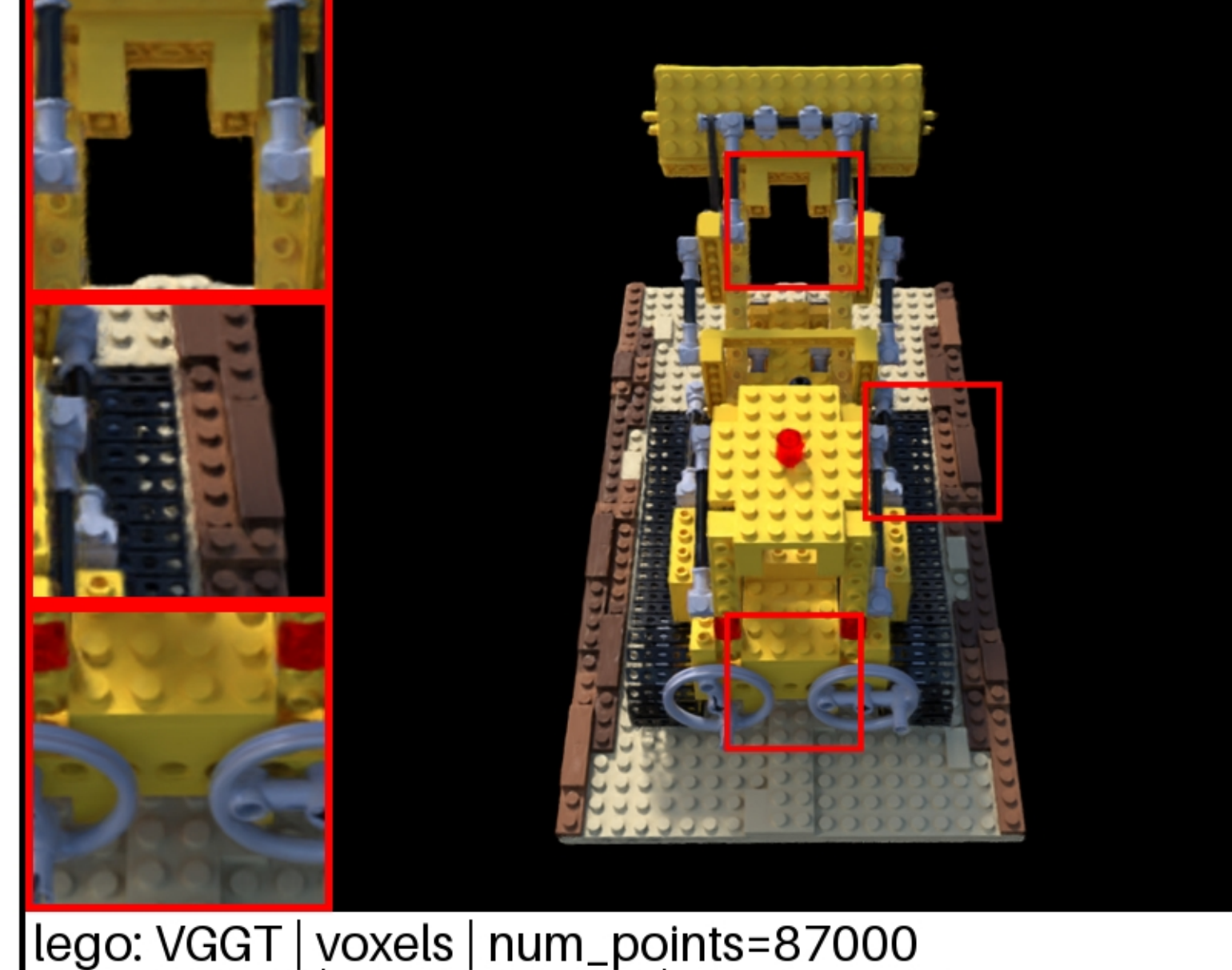
lego: VGGT | voxels | num_points=87000 PSNR: 20.56 | LPIPS: 0.0959 | SSIM: 0.7731
