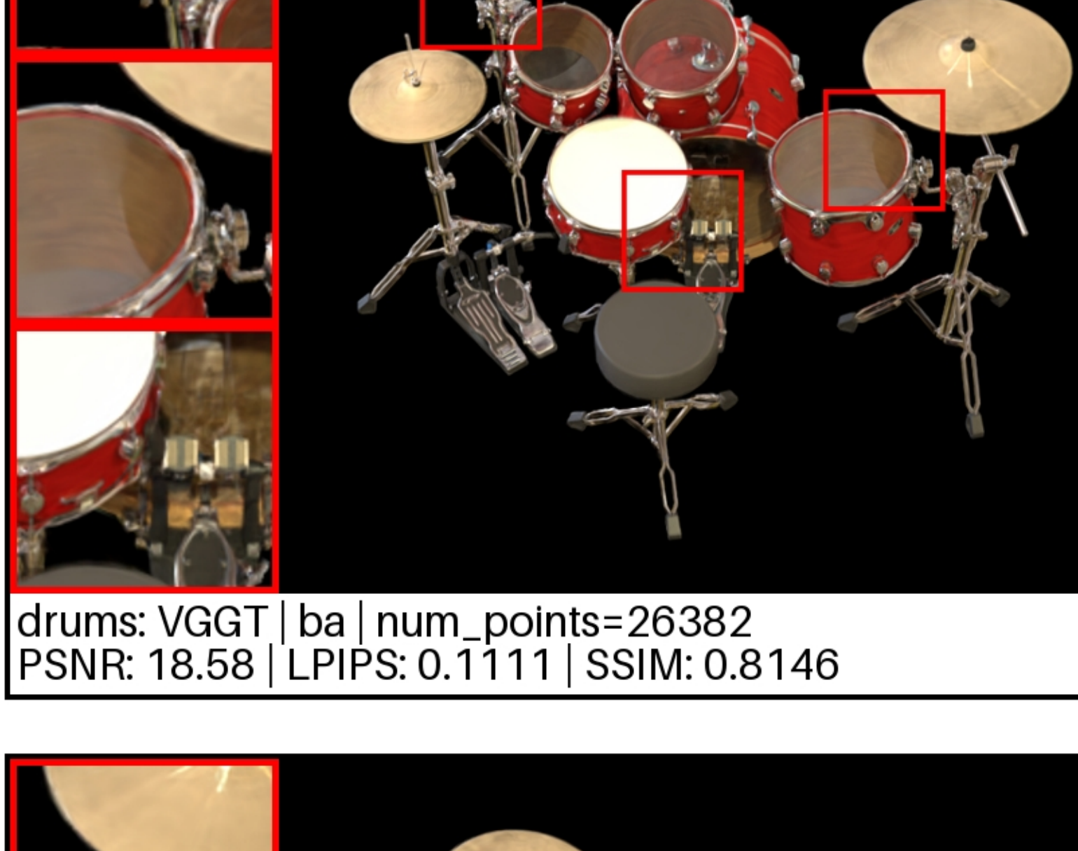
drums: VGGT | ba | num_points=26382 PSNR: 18.58 | LPIPS: 0.1111 | SSIM: 0.8146
