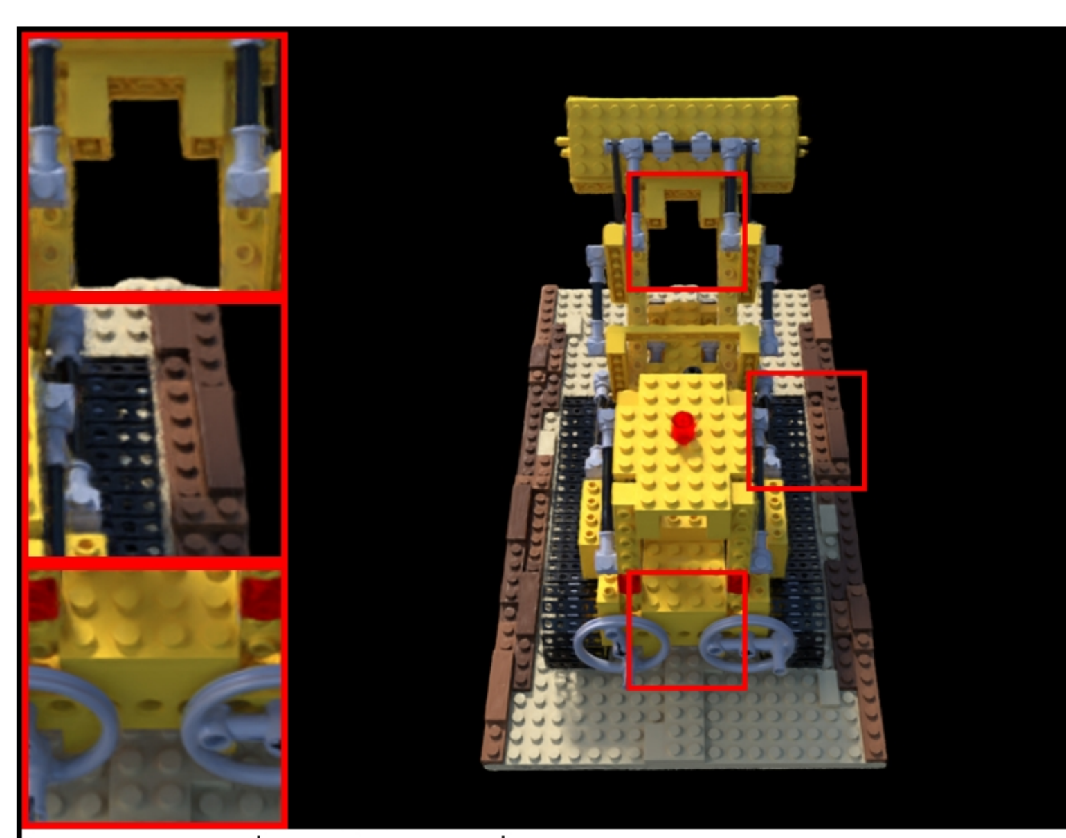
lego: VGGT | confidence | num_points=87000 PSNR: 20.61 | LPIPS: 0.0946 | SSIM: 0.7749
