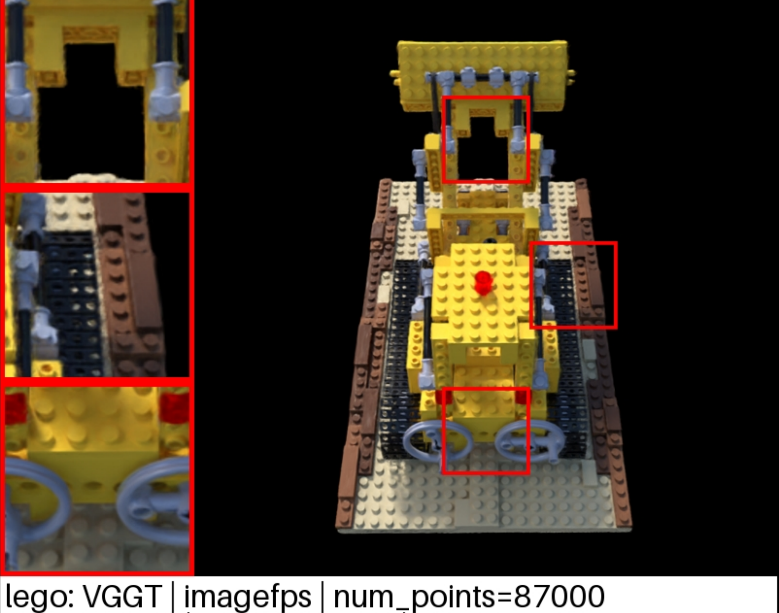
lego: VGGT | imagefps | num_points=87000 PSNR: 20.58 | LPIPS: 0.0959 | SSIM: 0.7741
