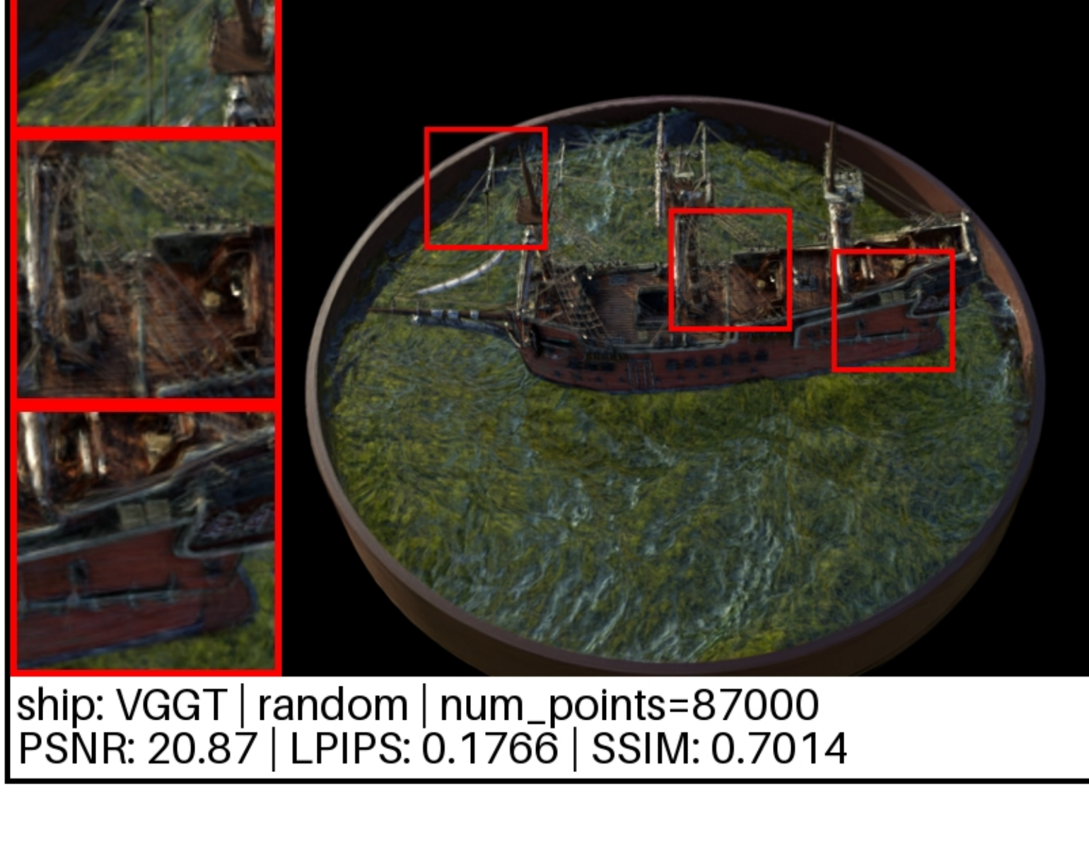
ship: VGGT | random | num_points=87000 PSNR: 20.87 | LPIPS: 0.1766 | SSIM: 0.7014
