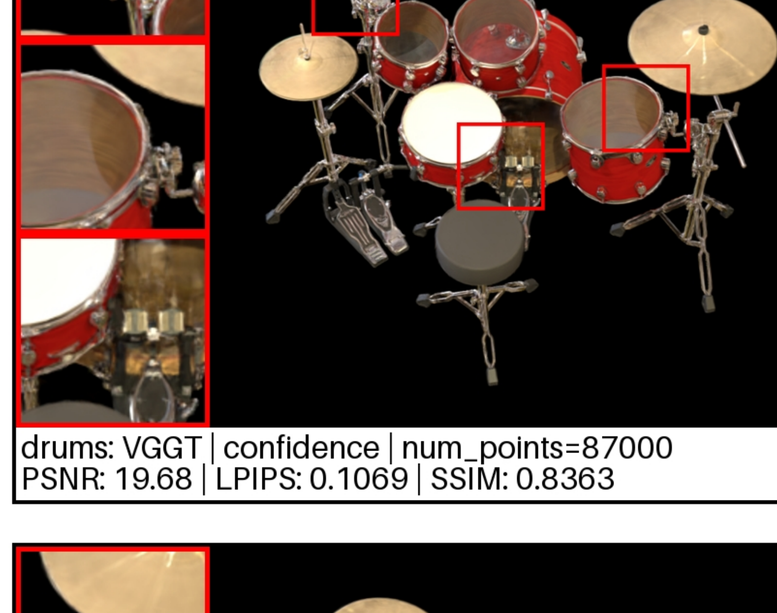
drums: VGGT | confidence | num_points=87000 PSNR: 19.68 | LPIPS: 0.1069 | SSIM: 0.8363
