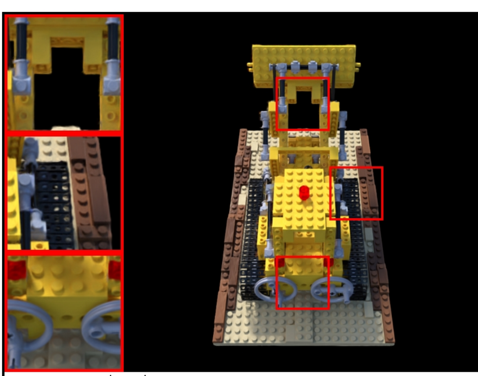
lego: VGGT | ba | num_points=27774 PSNR: 22.97 | LPIPS: 0.0746 | SSIM: 0.8368
