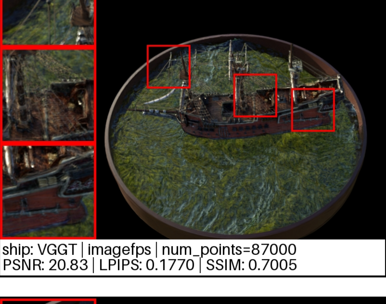
ship: VGGT | imagefps | num_points=87000 PSNR: 20.83 | LPIPS: 0.1770 | SSIM: 0.7005
