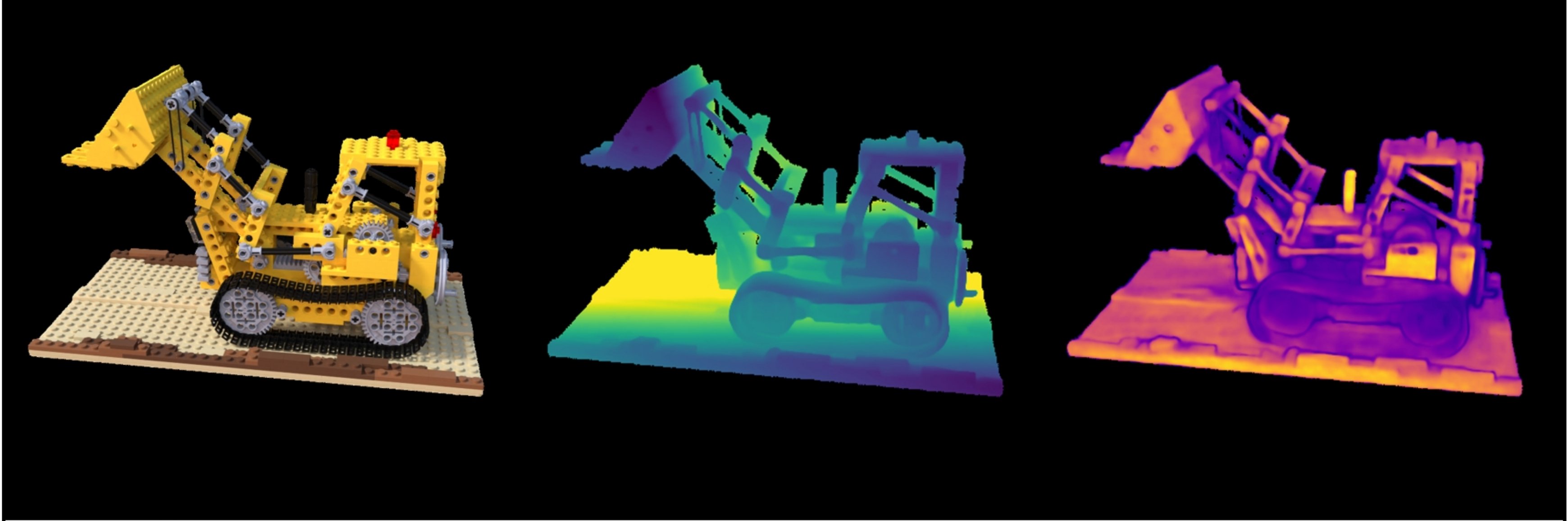
lego: VGGT | | num_images=7 Original | Depth (max=1.22) | Confidence (max=72.63)
