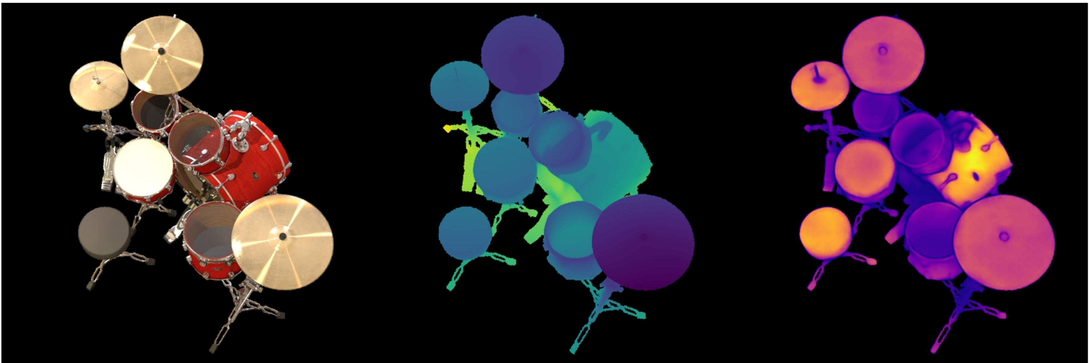
drums: VGGT | | num_images=7 Original | Depth (max=1.22) | Confidence (max=196.96)
