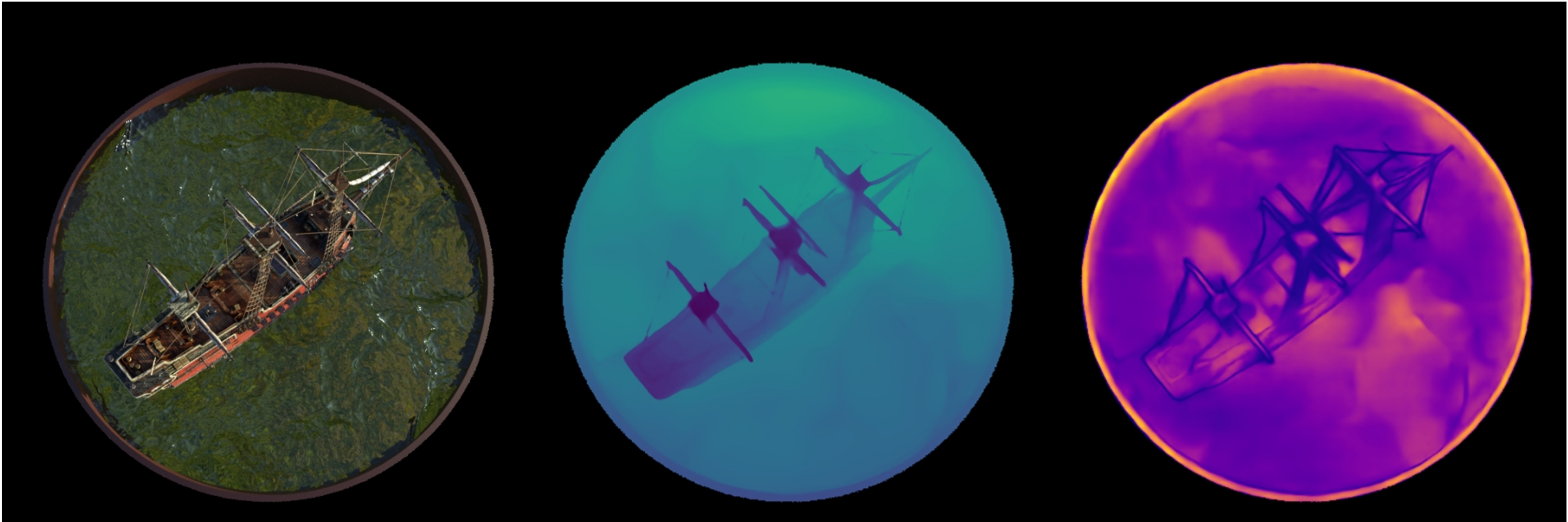
ship: VGGT | | num_images=7 Original | Depth (max=1.09) | Confidence (max=102.89)
