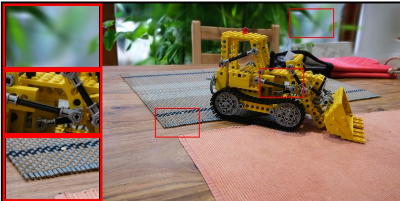
kitchen: Combined | COLMAP Cams | Both Pcds | confide PSNR: 22.61 | LPIPS: 0.1249 | SSIM: 0.5725
