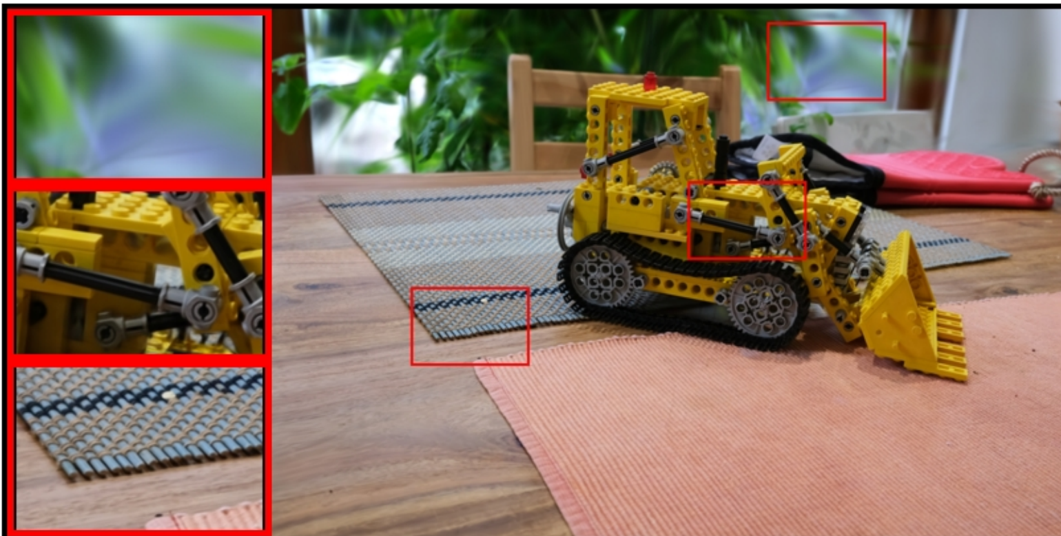
kitchen: COLMAP | | | PSNR: 22.44 | LPIPS: 0.1272 | SSIM: 0.5514
