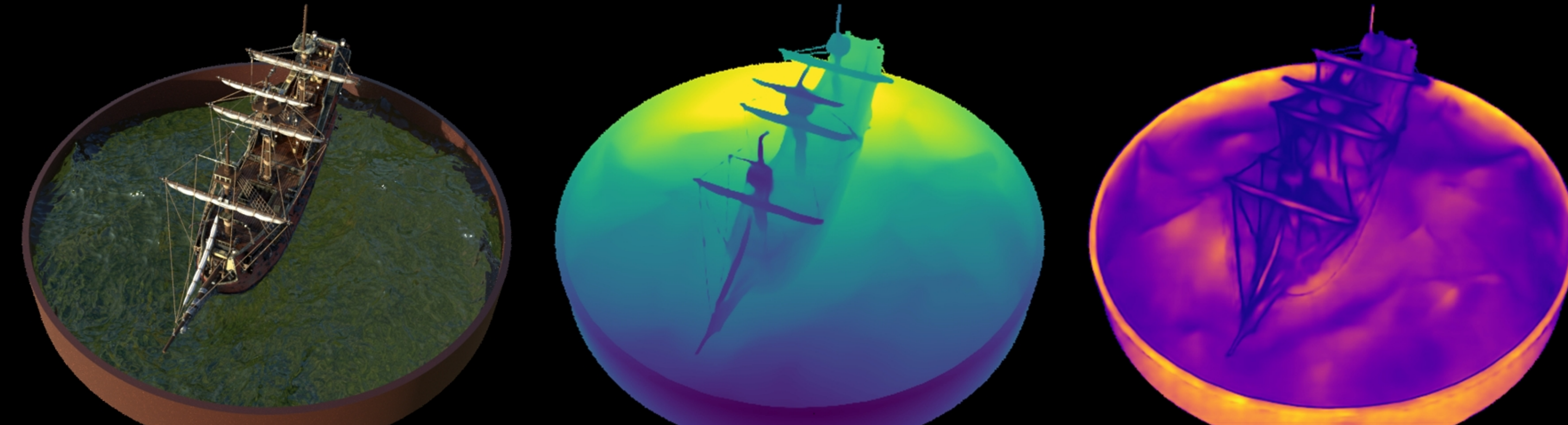
ship: Combined | COLMAP Cams | Both Pcds | confidence Original | Depth (max=6.66) | Confidence (max=793.41)
