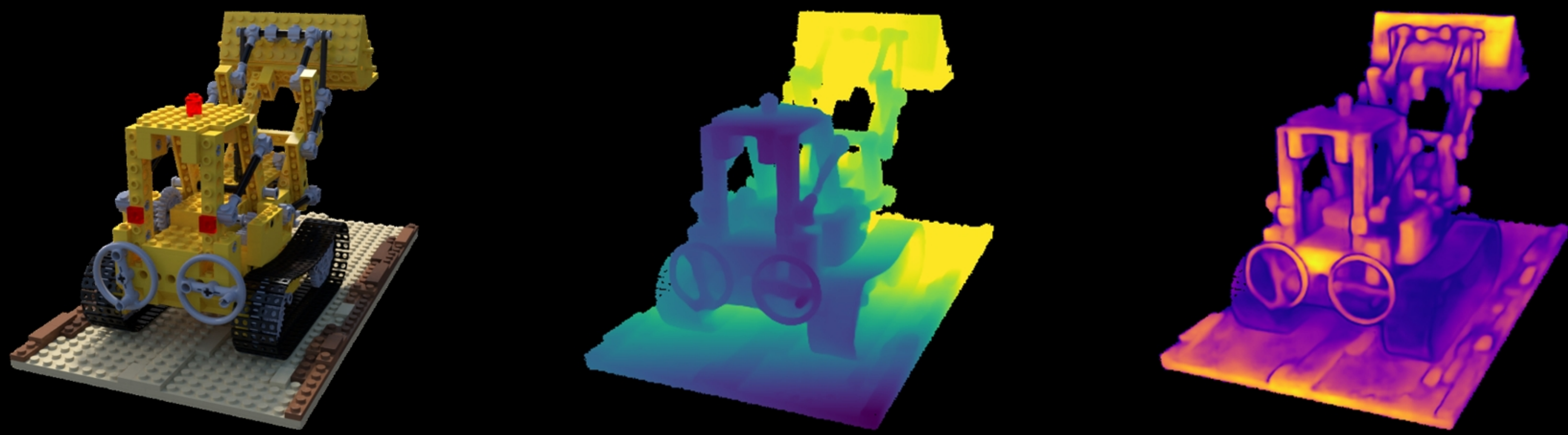
lego: Combined | COLMAP Cams | Both Pcds | confidence Original | Depth (max=5.88) | Confidence (max=713.75)
