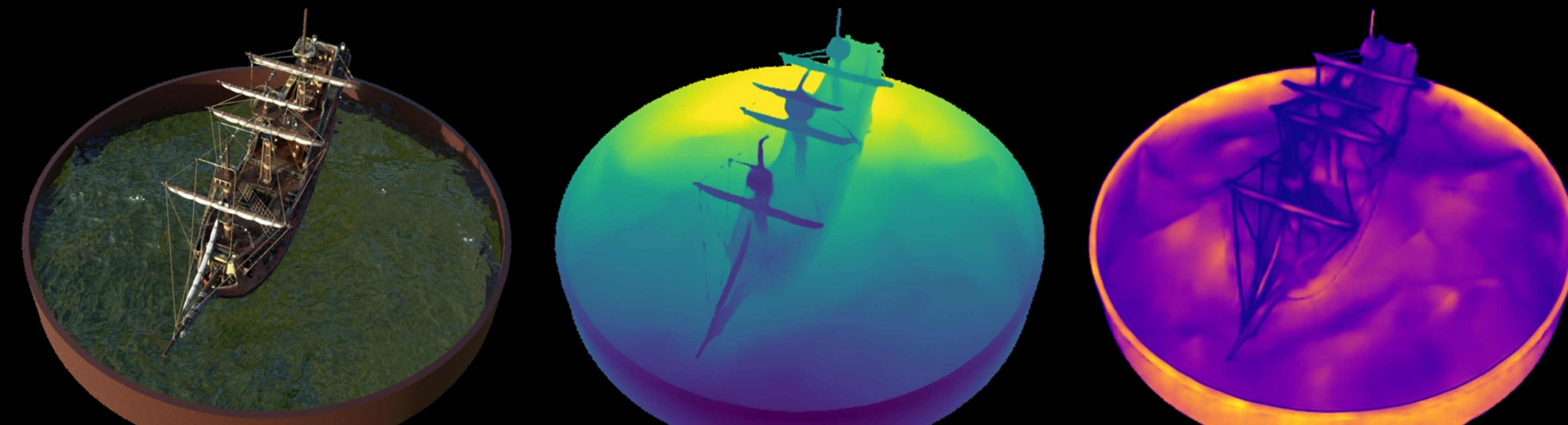
ship: VGGT | | confidence Original | Depth (max=1.23) | Confidence (max=146.85)
