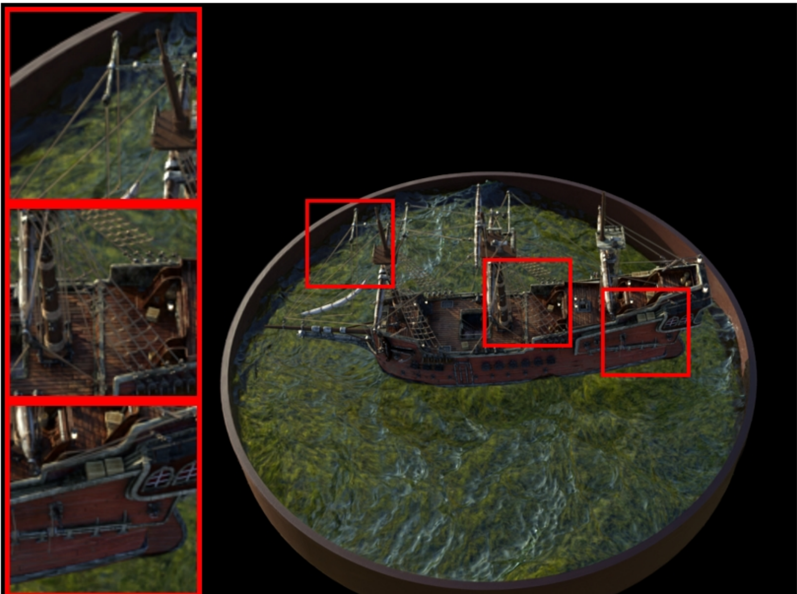
ship: VGGT | | confidence PSNR: 22.84 | LPIPS: 0.1290 | SSIM: 0.7482
