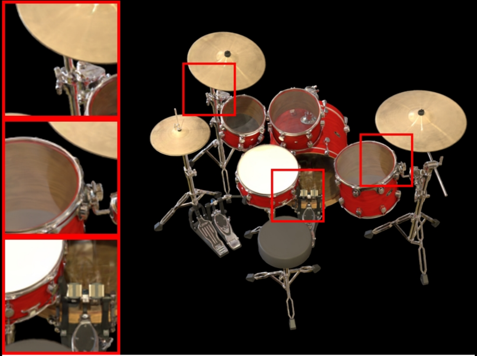
drums: VGGT | | confidence PSNR: 20.87 | LPIPS: 0.0852 | SSIM: 0.8683
