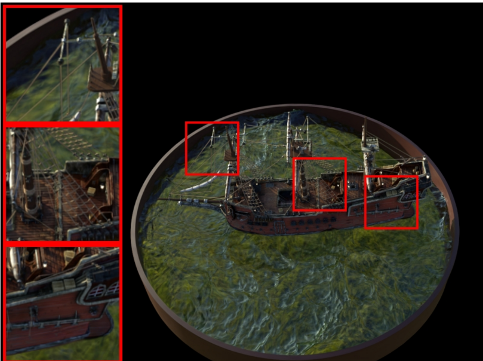
ship: COLMAP | | | PSNR: 22.68 | LPIPS: 0.1422 | SSIM: 0.7593
