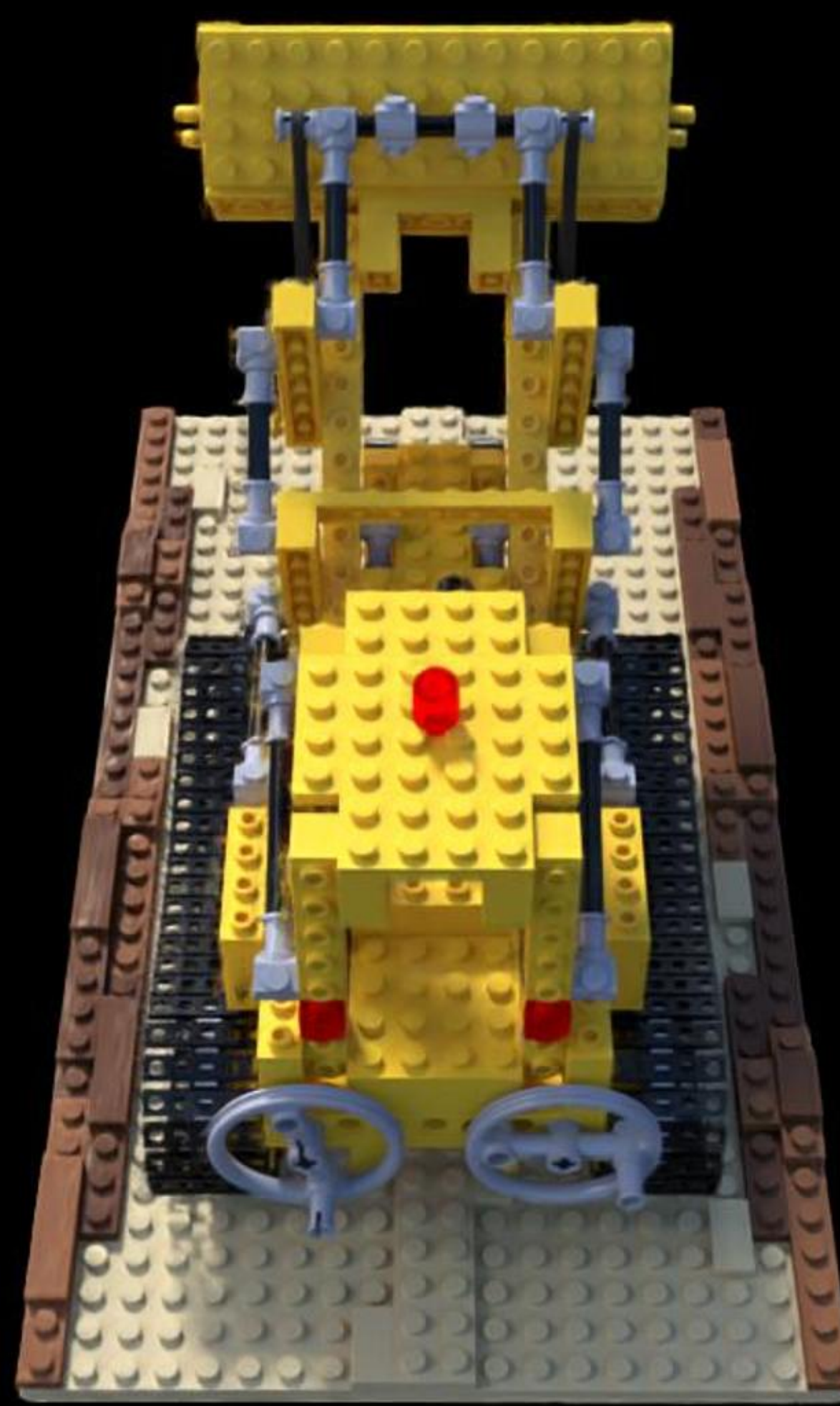
Config: VGGT | ba | num_points=30396 PSNR: 20.45 | LPIPS: 0.0953 | SSIM: 0.7806
