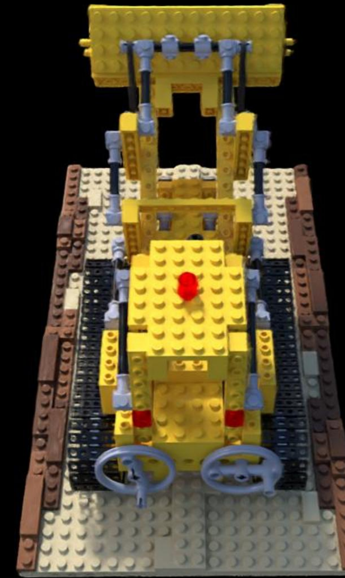
Config: VGGT | confidence | num_points=87000 PSNR: 19.91 | LPIPS: 0.1063 | SSIM: 0.7480
