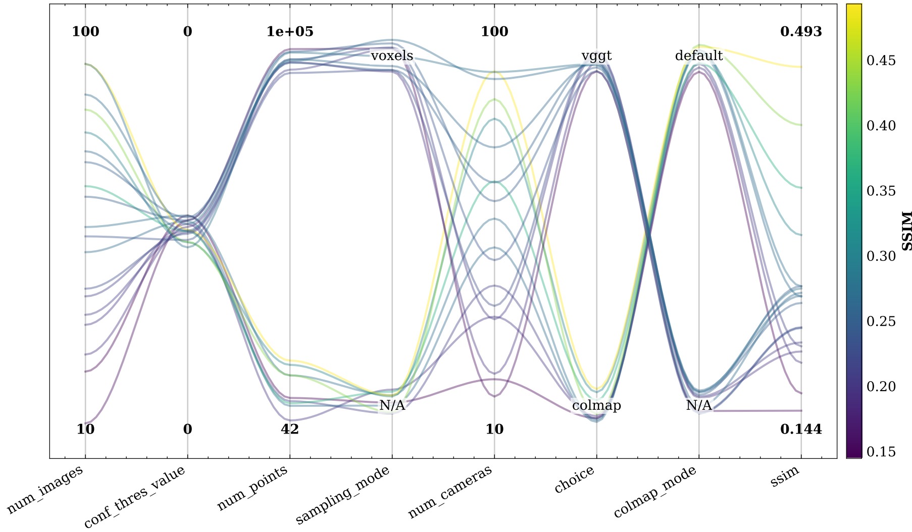
Parallel Coordinate Plot: Parameters vs SSIM
