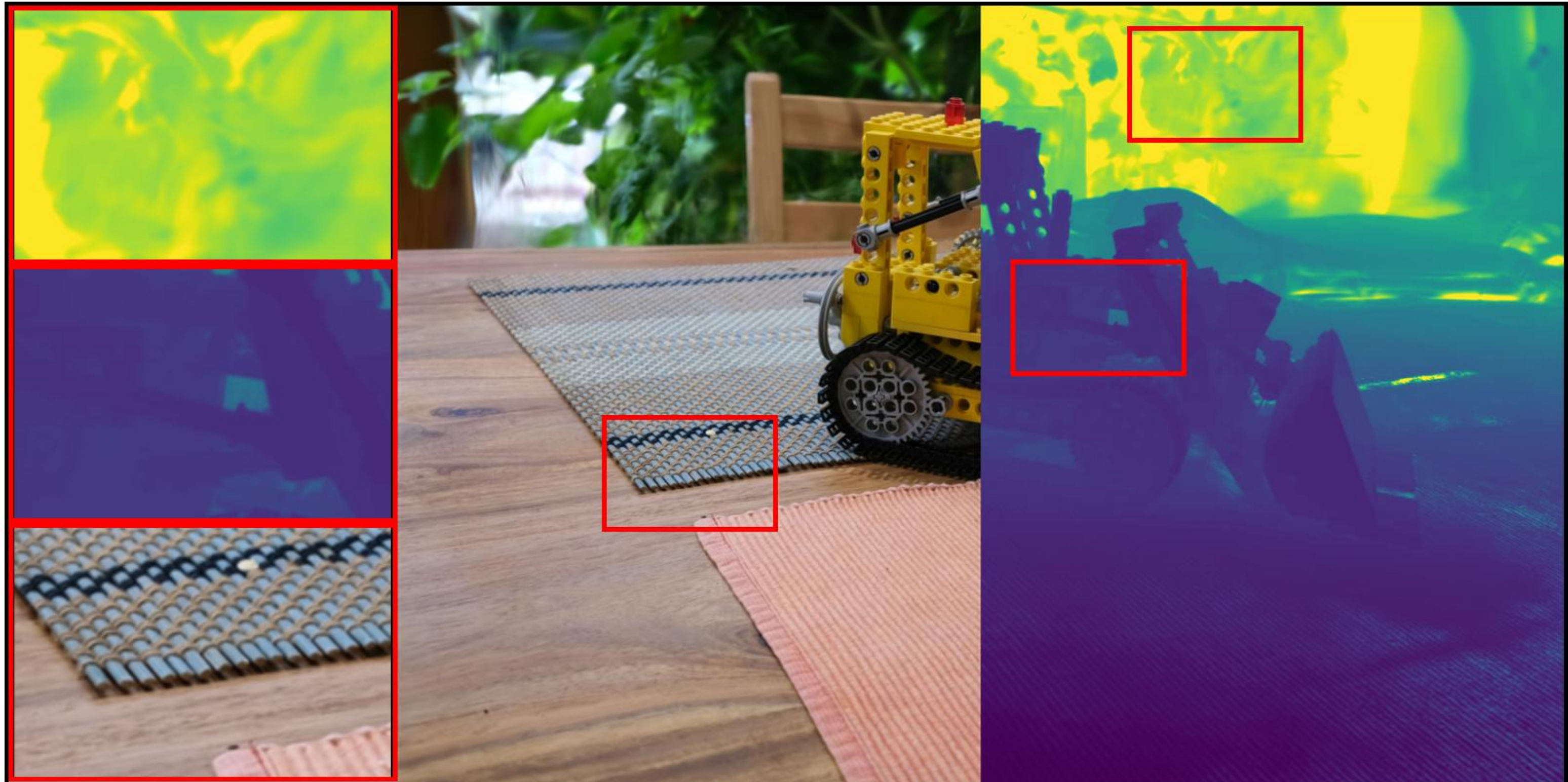
kitchen: VGGT | closer | depth_lambda=0.1 PSNR: 26.16 | LPIPS: 0.1273 | SSIM: 0.8917
