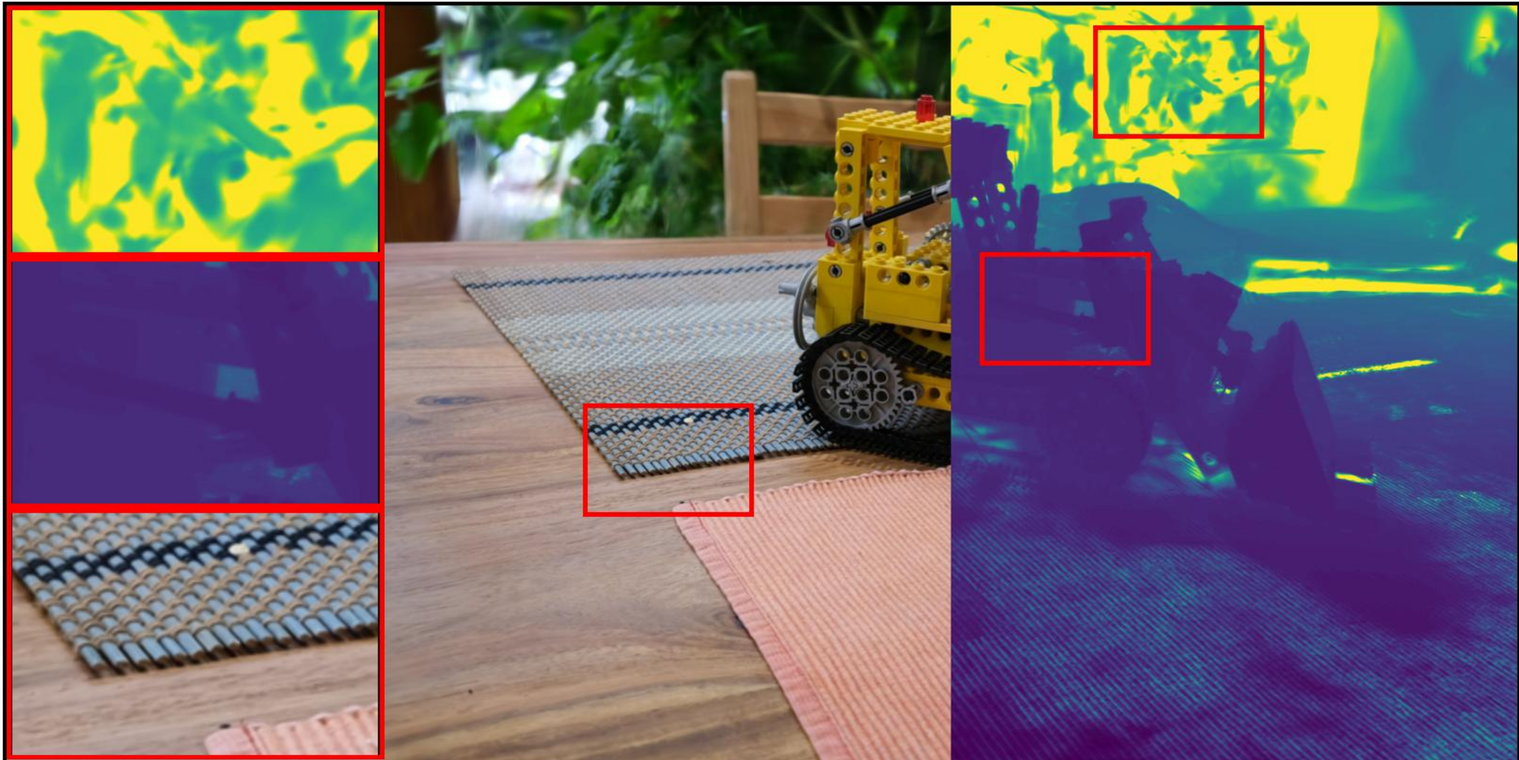
kitchen: VGGT | closer | depth_lambda=0.01 PSNR: 25.73 | LPIPS: 0.1298 | SSIM: 0.8879
