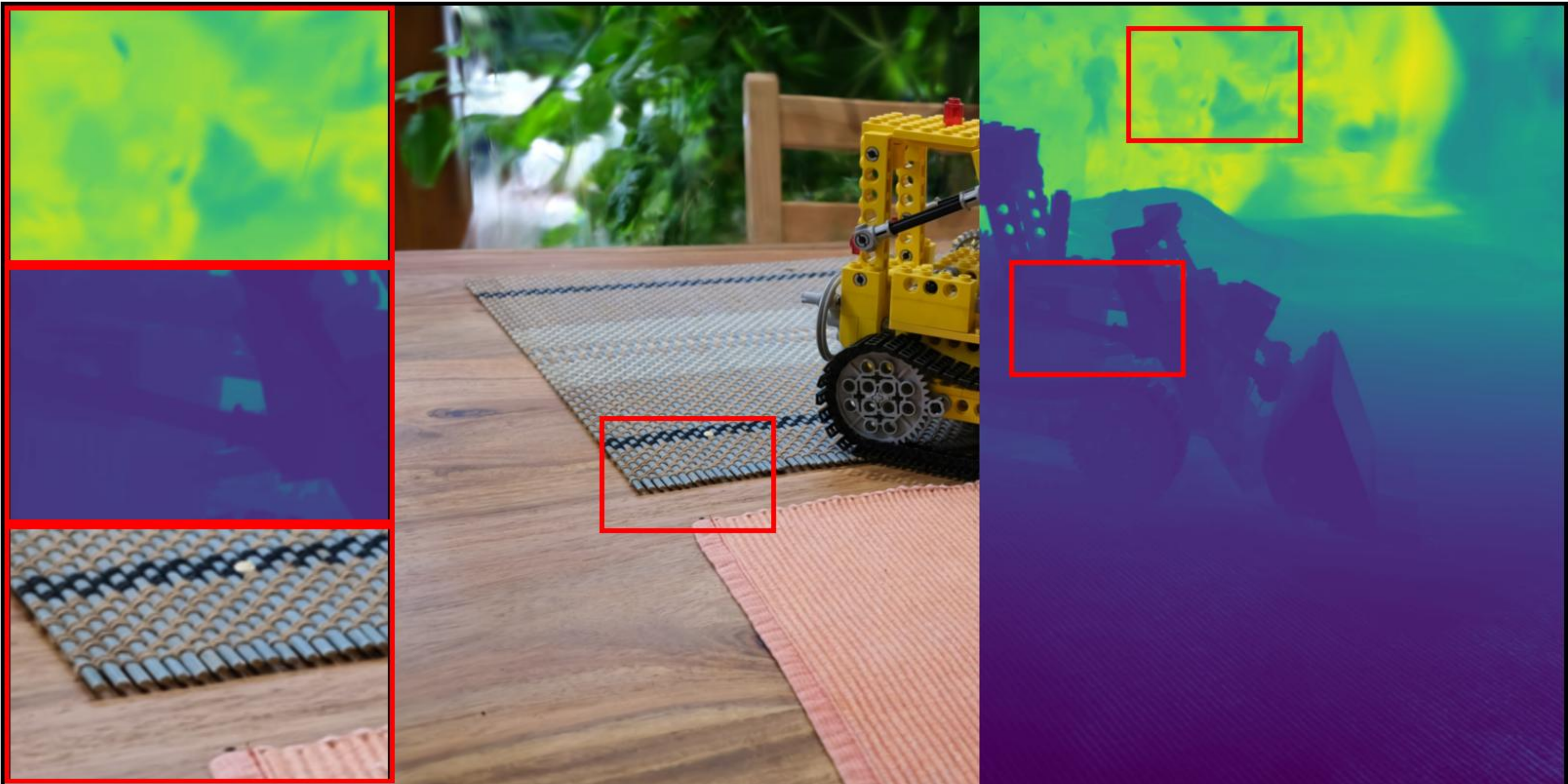
kitchen: VGGT | | depth_lambda=0.0 PSNR: 25.89 | LPIPS: 0.1295 | SSIM: 0.8895
