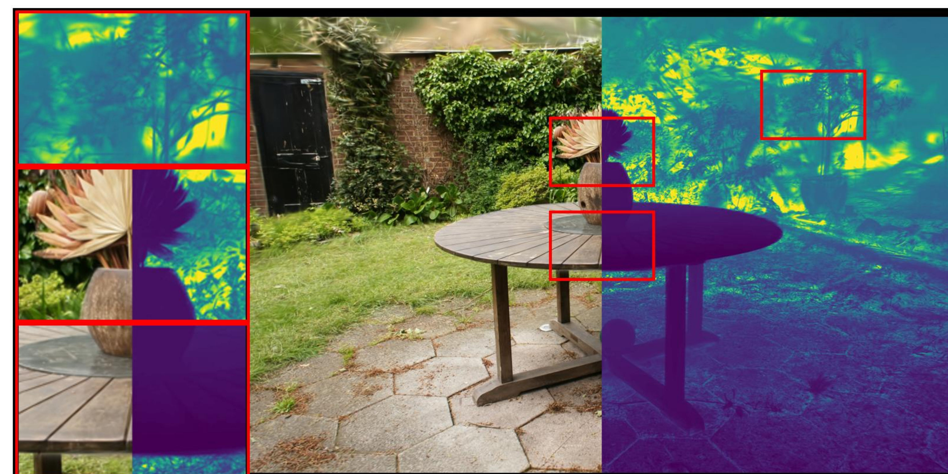
garden: VGGT | depth_lambda=1.0 PSNR: 19.54 | LPIPS: 0.3319 | SSIM: 0.3608
