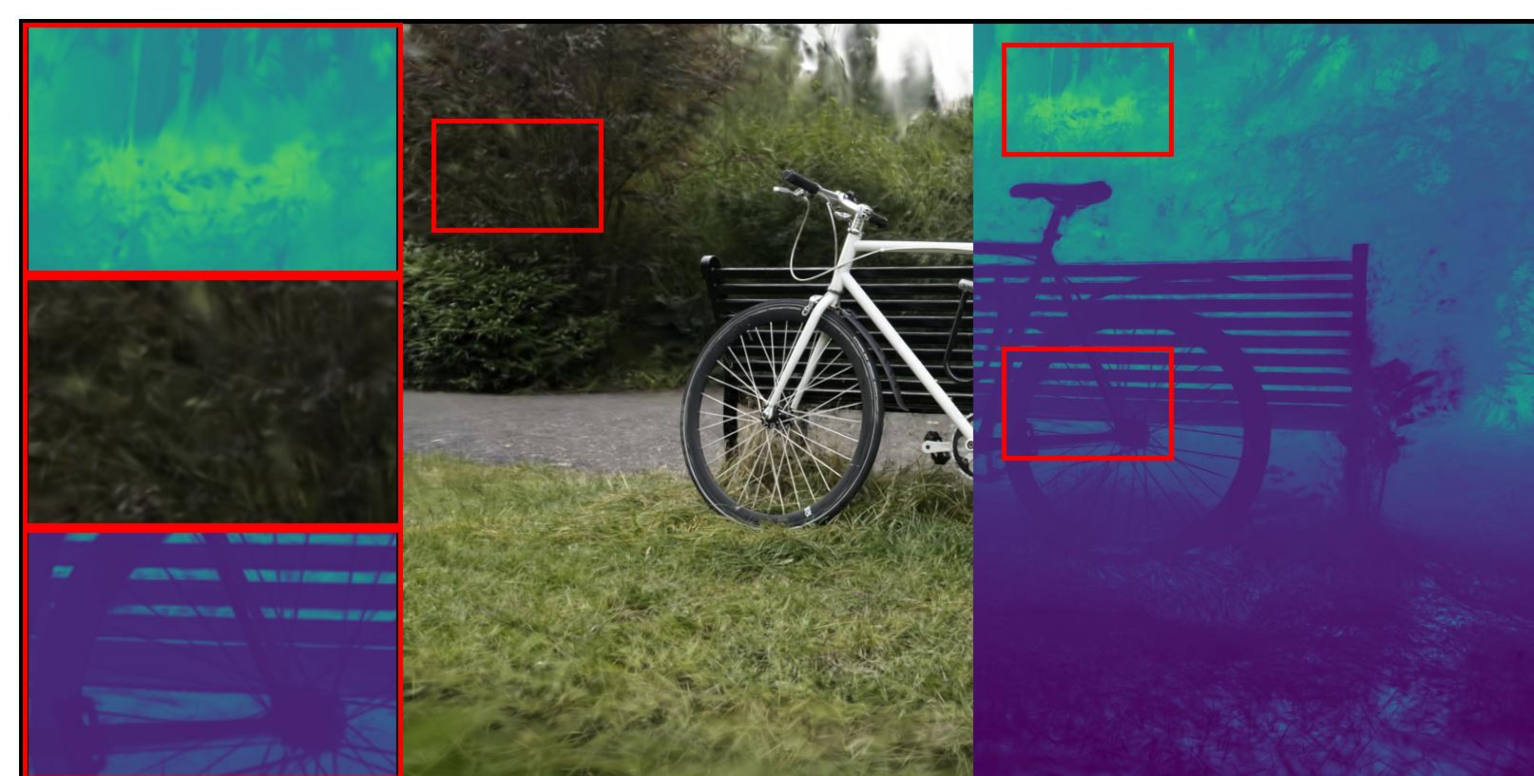
bicycle: VGGT | depth_lambda=0.0 PSNR: 17.38 | LPIPS: 0.3378 | SSIM: 0.2679
