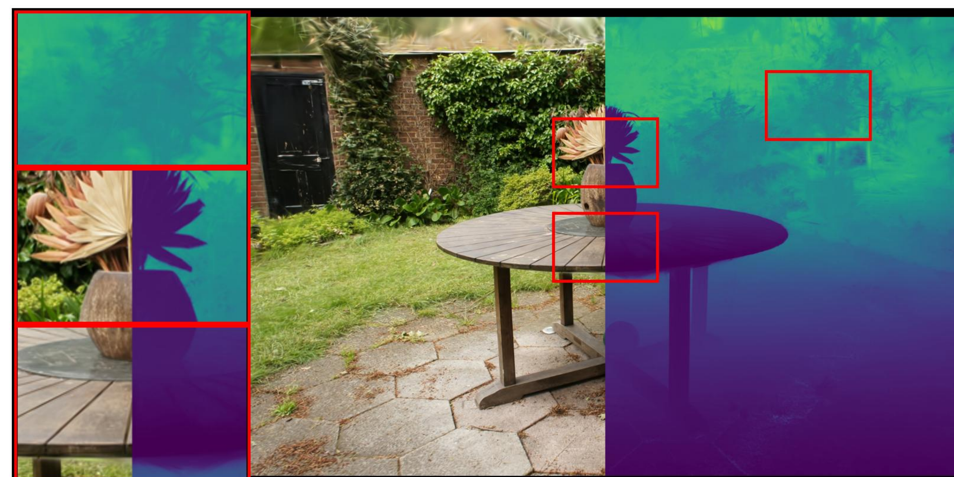
garden: VGGT | depth_lambda=0.0 PSNR: 19.35 | LPIPS: 0.3378 | SSIM: 0.3664
