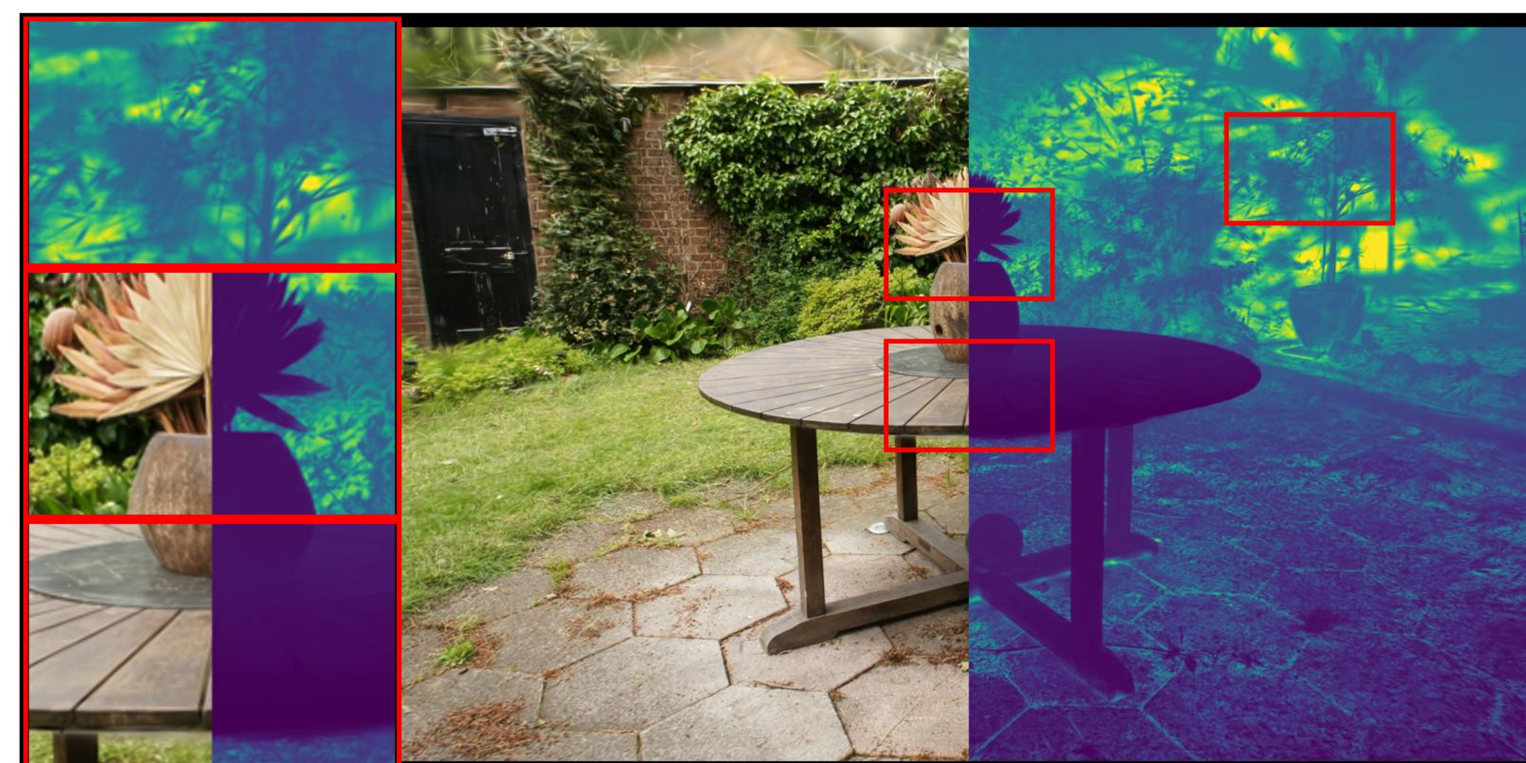
garden: VGGT | depth_lambda=0.1 PSNR: 19.50 | LPIPS: 0.3344 | SSIM: 0.3649
