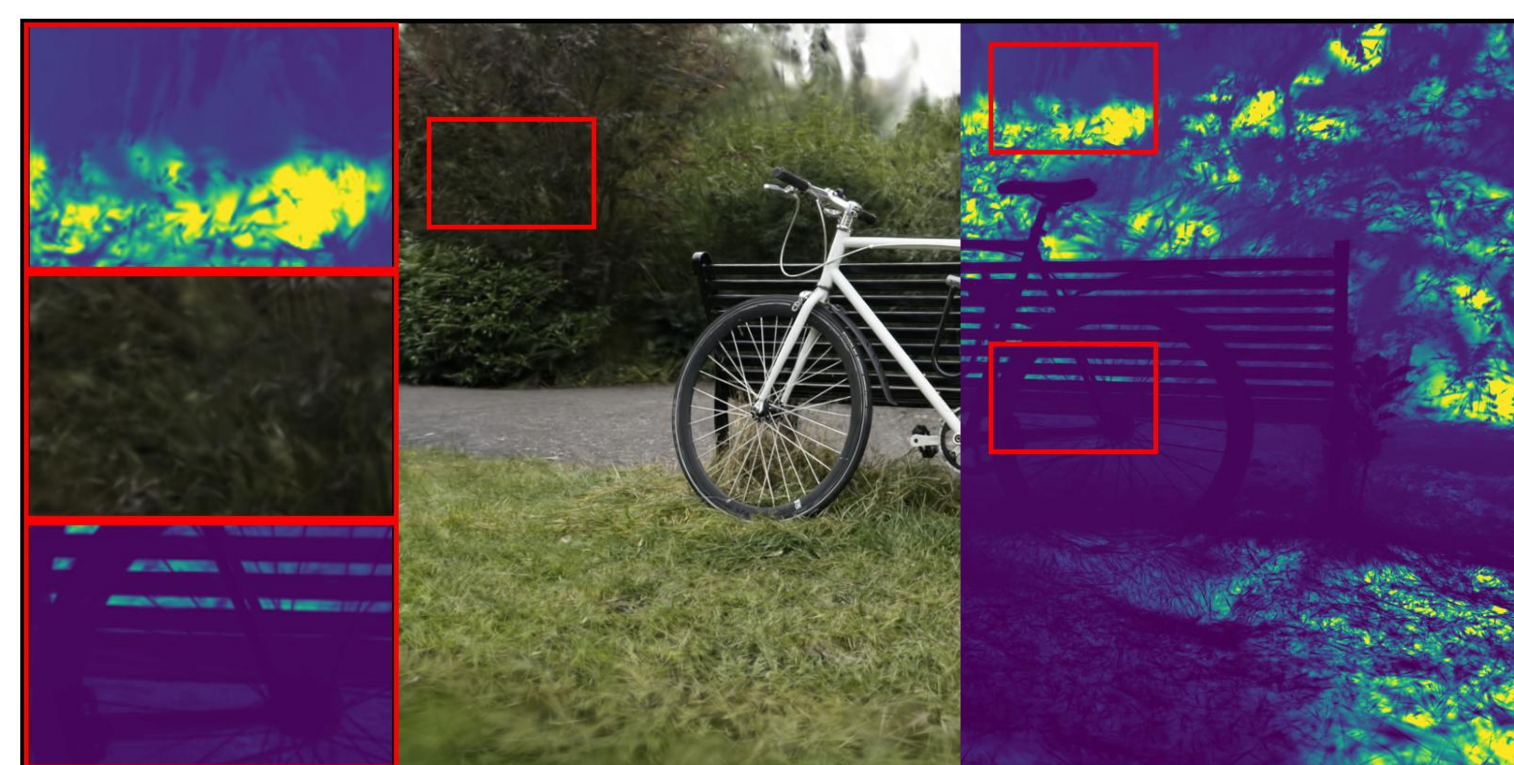
bicycle: VGGT | depth_lambda=0.01 PSNR: 17.44 | LPIPS: 0.3352 | SSIM: 0.2689
