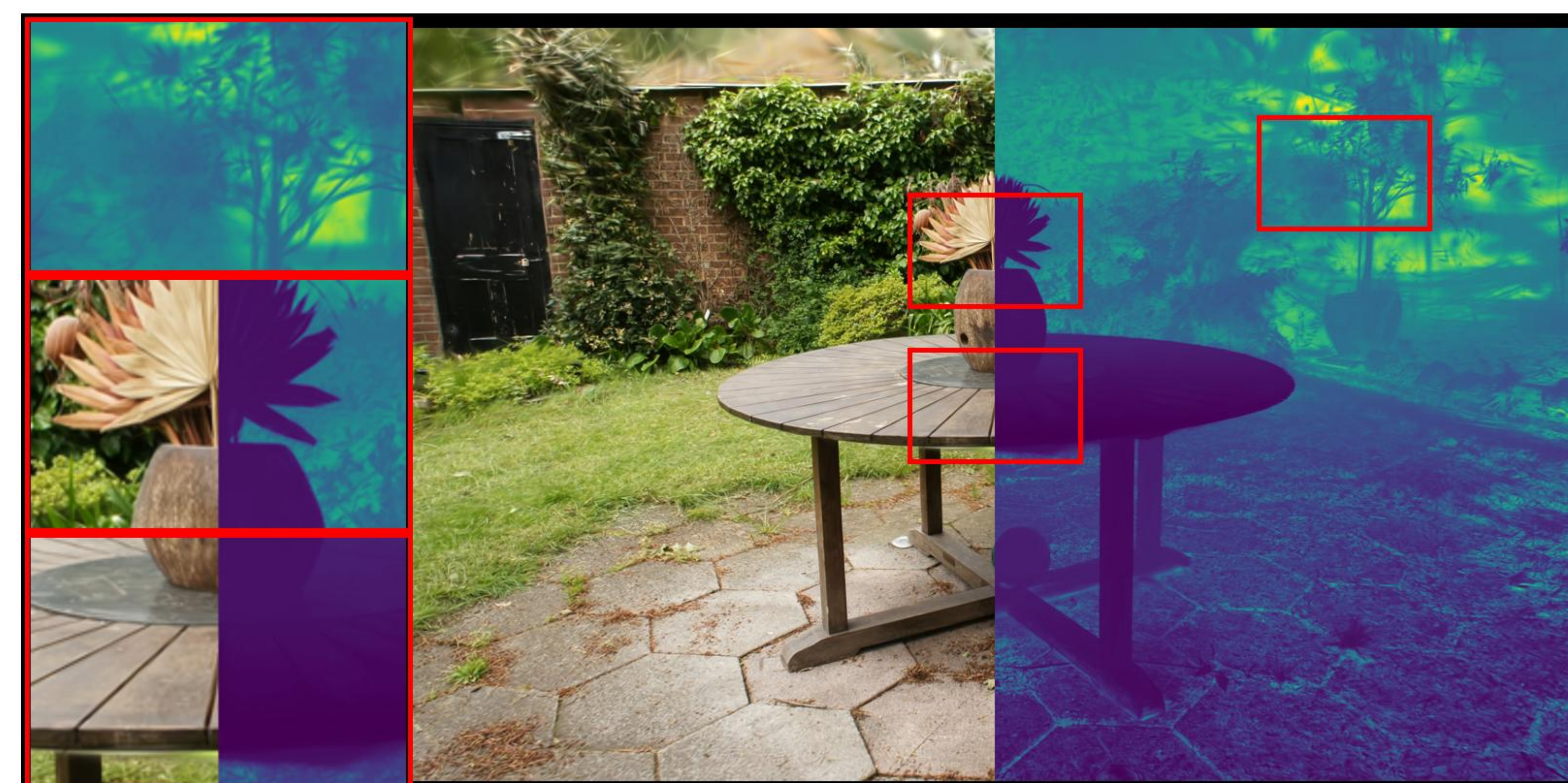
garden: VGGT | depth_lambda=0.01 PSNR: 19.51 | LPIPS: 0.3351 | SSIM: 0.3669
