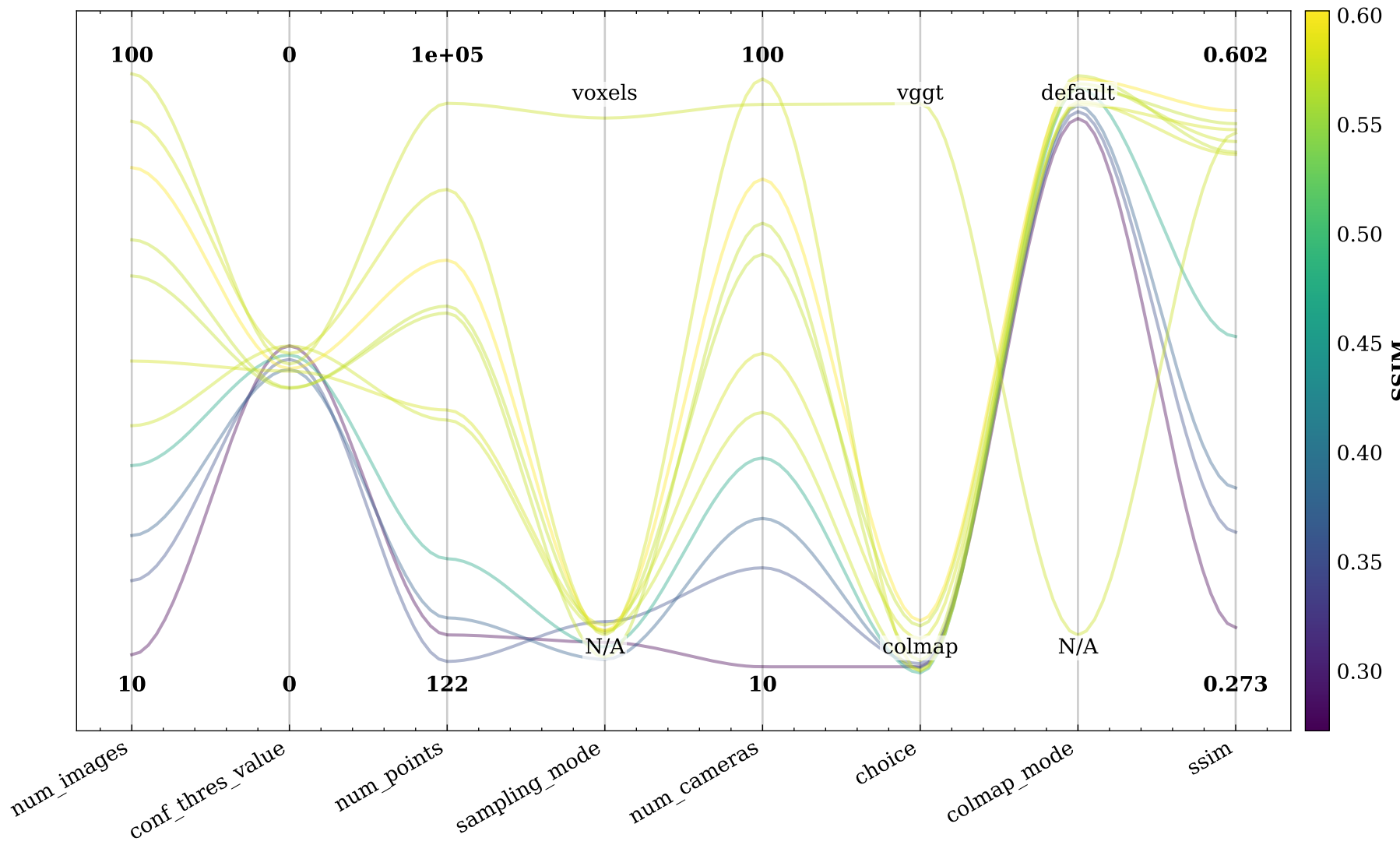
Parallel Coordinate Plot: Parameters vs SSIM
