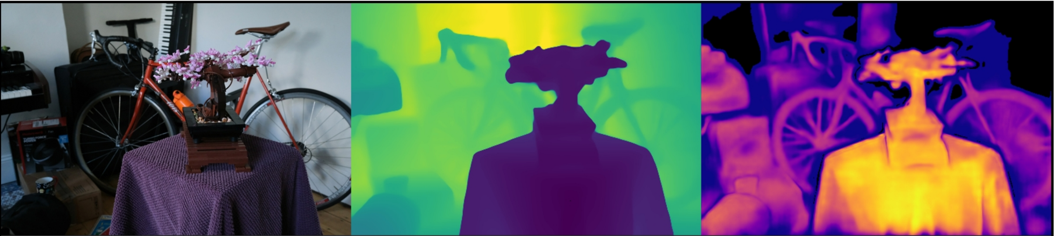
bonsai: VGGT | minfarthestpose | num_images=100 Original | Depth (max=2.16) | Confidence (max=5.62)
