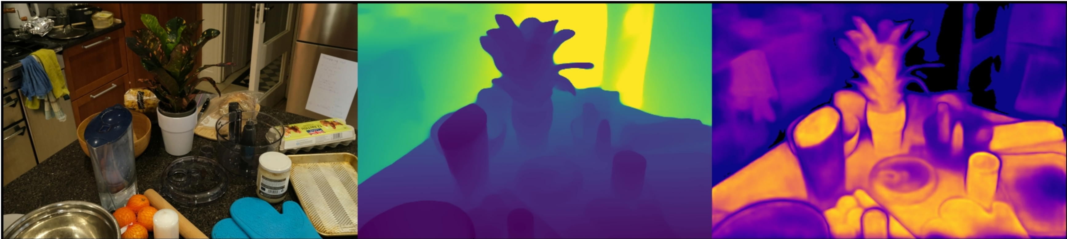
counter: VGGT | farthestpose | num_images=100 Original | Depth (max=2.88) | Confidence (max=15.71)
