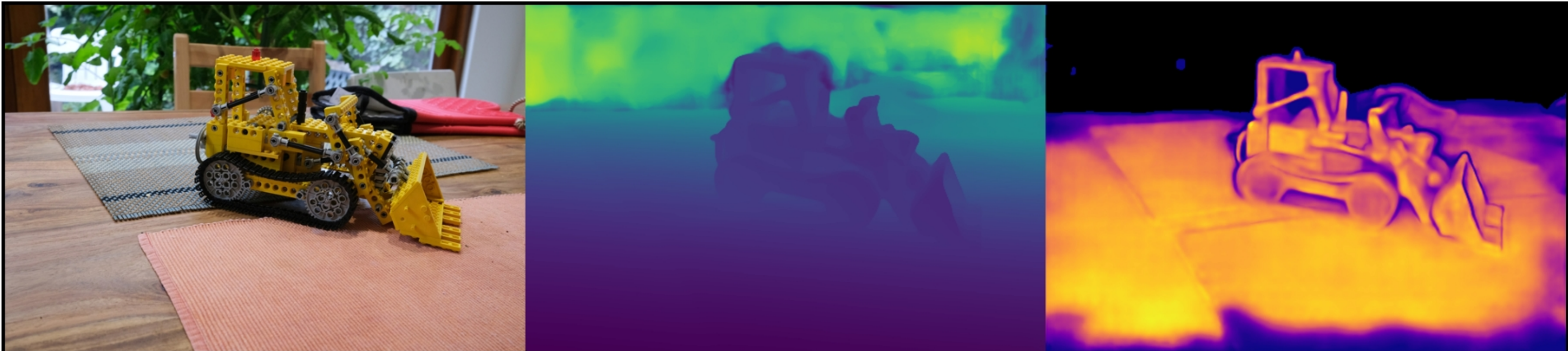
kitchen: VGGT | farthestpose | num_images=100 Original | Depth (max=2.43) | Confidence (max=30.80)
