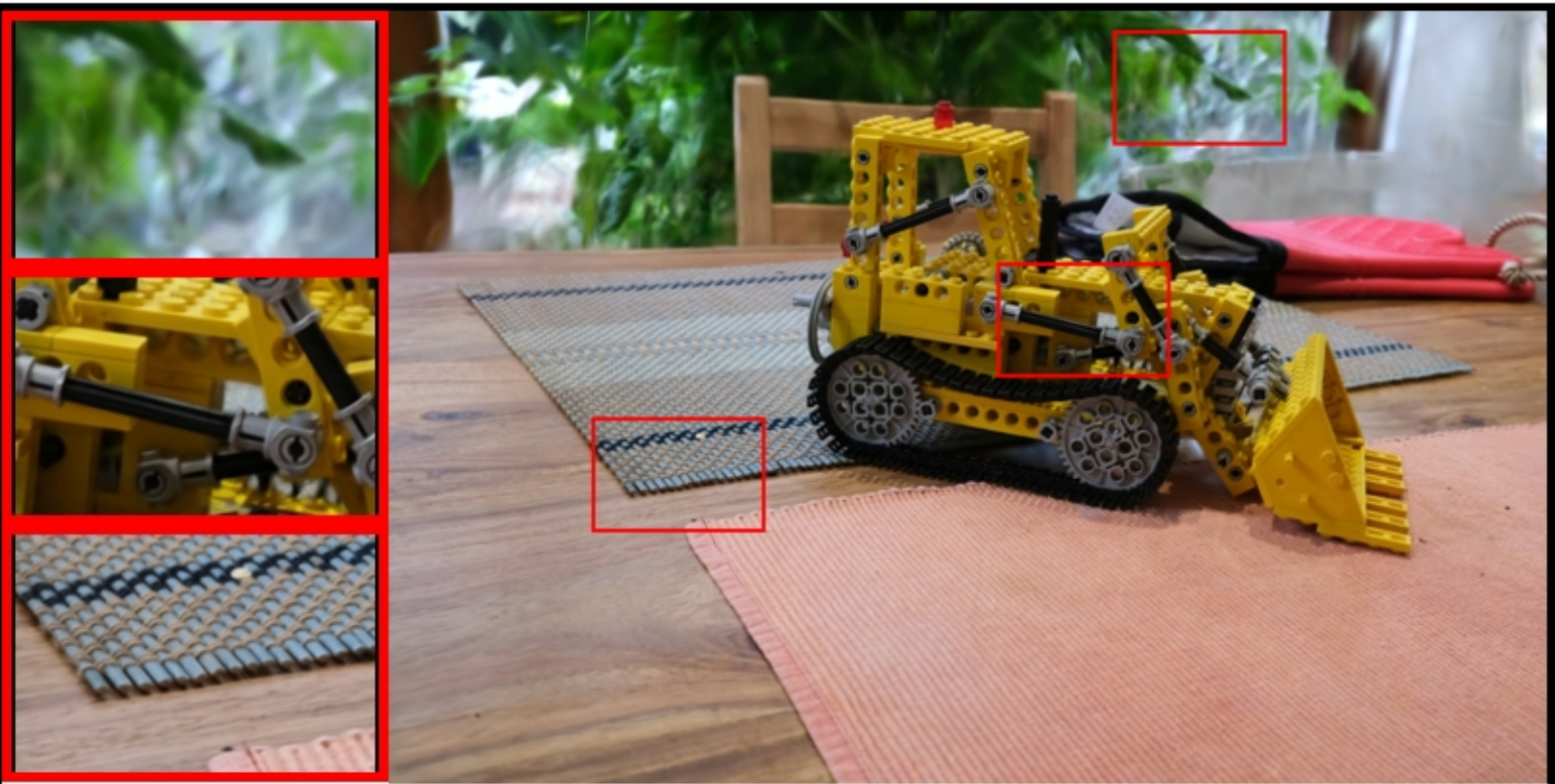
kitchen: VGGT | minfarthestpose | num_images=100 PSNR: 21.23 | LPIPS: 0.1559 | SSIM: 0.5311
