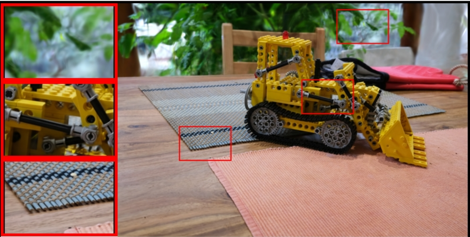
kitchen: VGGT | farthestpose | num_images=100 PSNR: 20.02 | LPIPS: 0.1764 | SSIM: 0.4138
