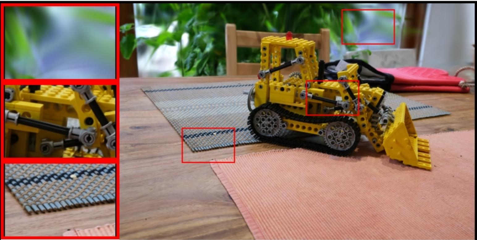
kitchen: COLMAP | minfarthestpose | num_images=100 PSNR: 22.44 | LPIPS: 0.1272 | SSIM: 0.5514
