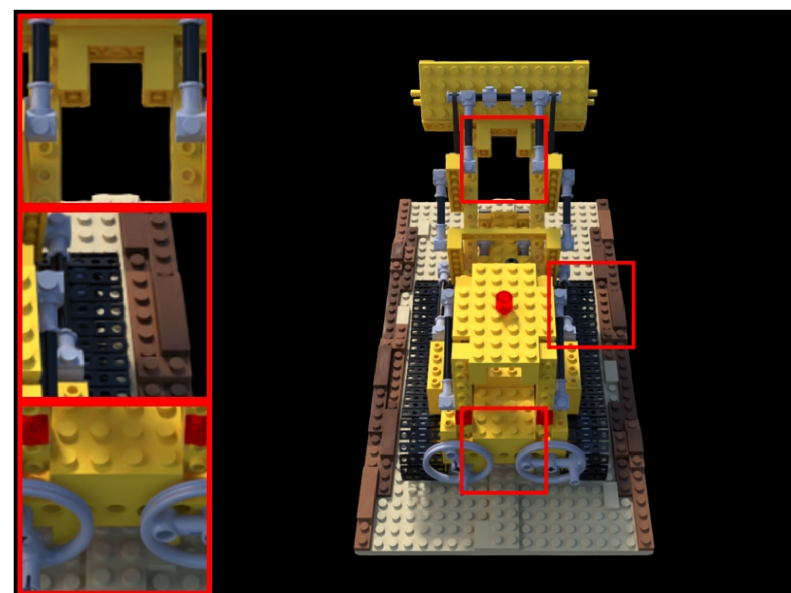
lego: COLMAP | minfarthestpose | num_images=87 PSNR: 24.42 | LPIPS: 0.0557 | SSIM: 0.8872
