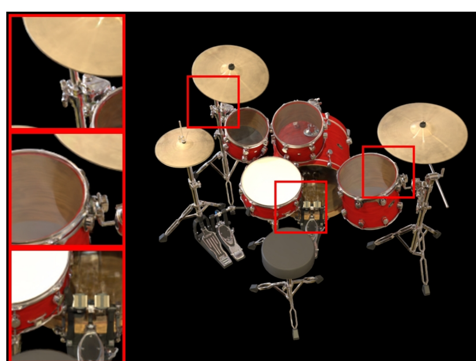
drums: VGGT | farthestpose | num_images=87 PSNR: 20.90 | LPIPS: 0.0848 | SSIM: 0.8690
