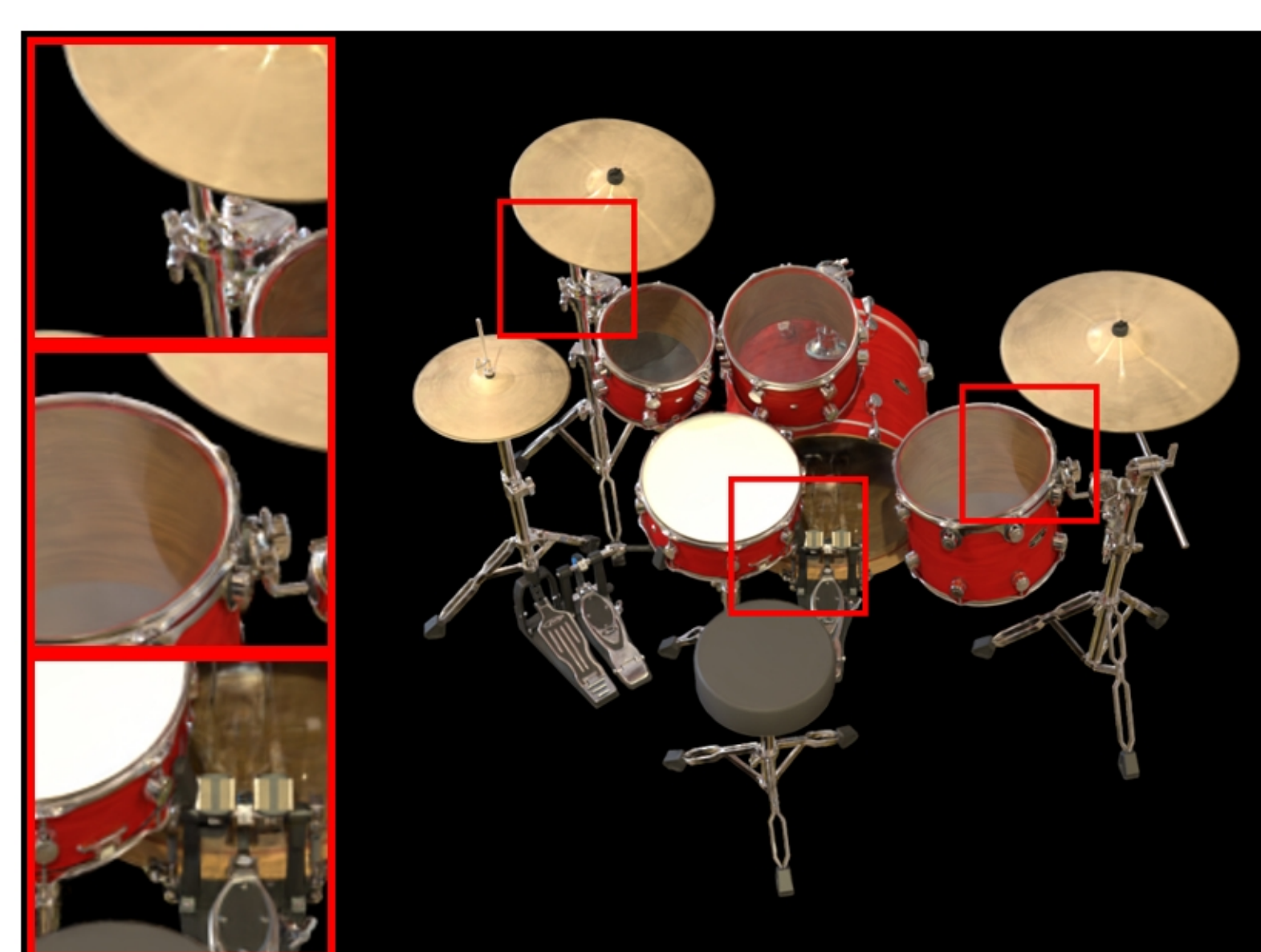
drums: VGGT | minfarthestpose | num_images=87 PSNR: 20.89 | LPIPS: 0.0847 | SSIM: 0.8688
