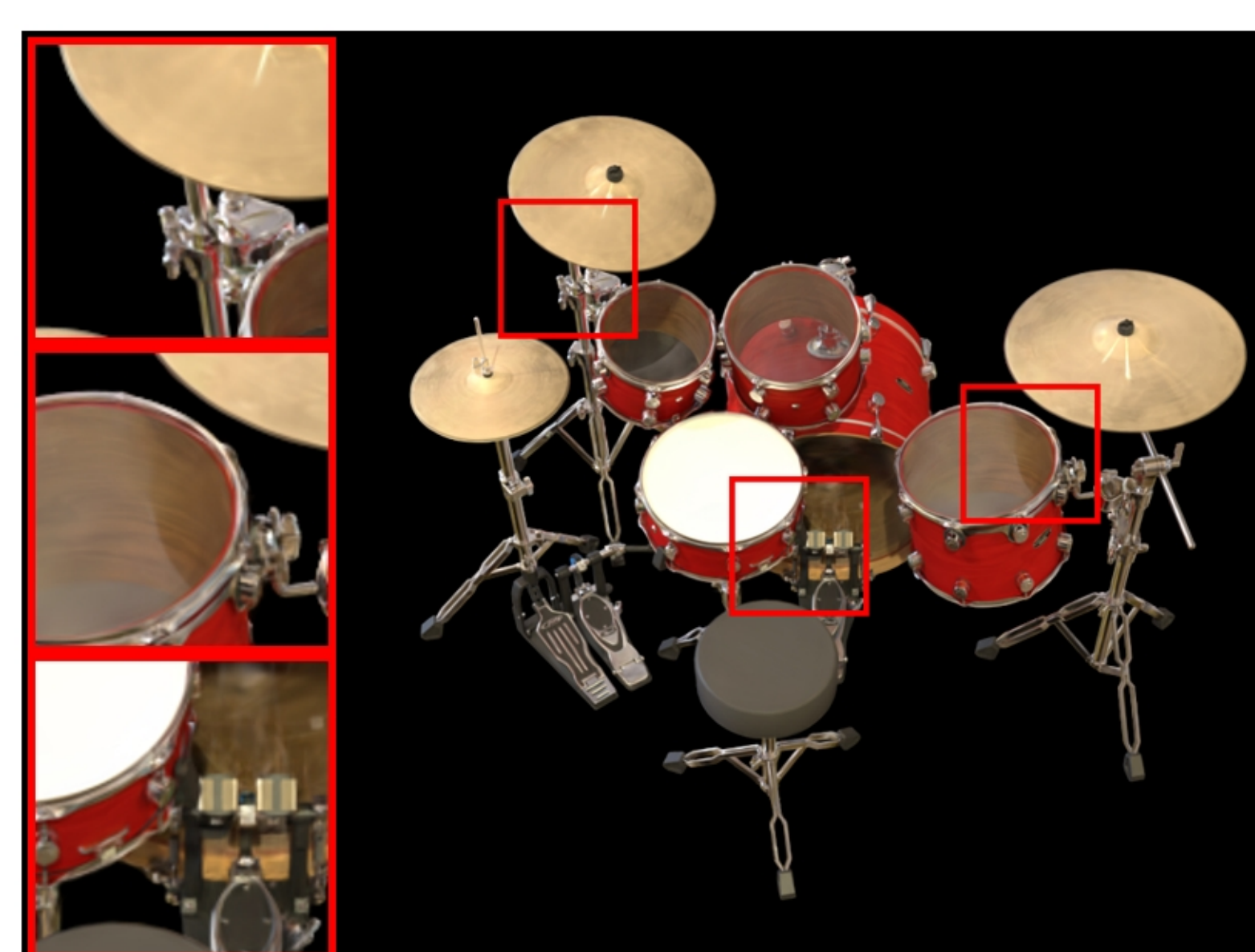
drums: COLMAP | minfarthestpose | num_images=87 PSNR: 22.95 | LPIPS: 0.0884 | SSIM: 0.9071
