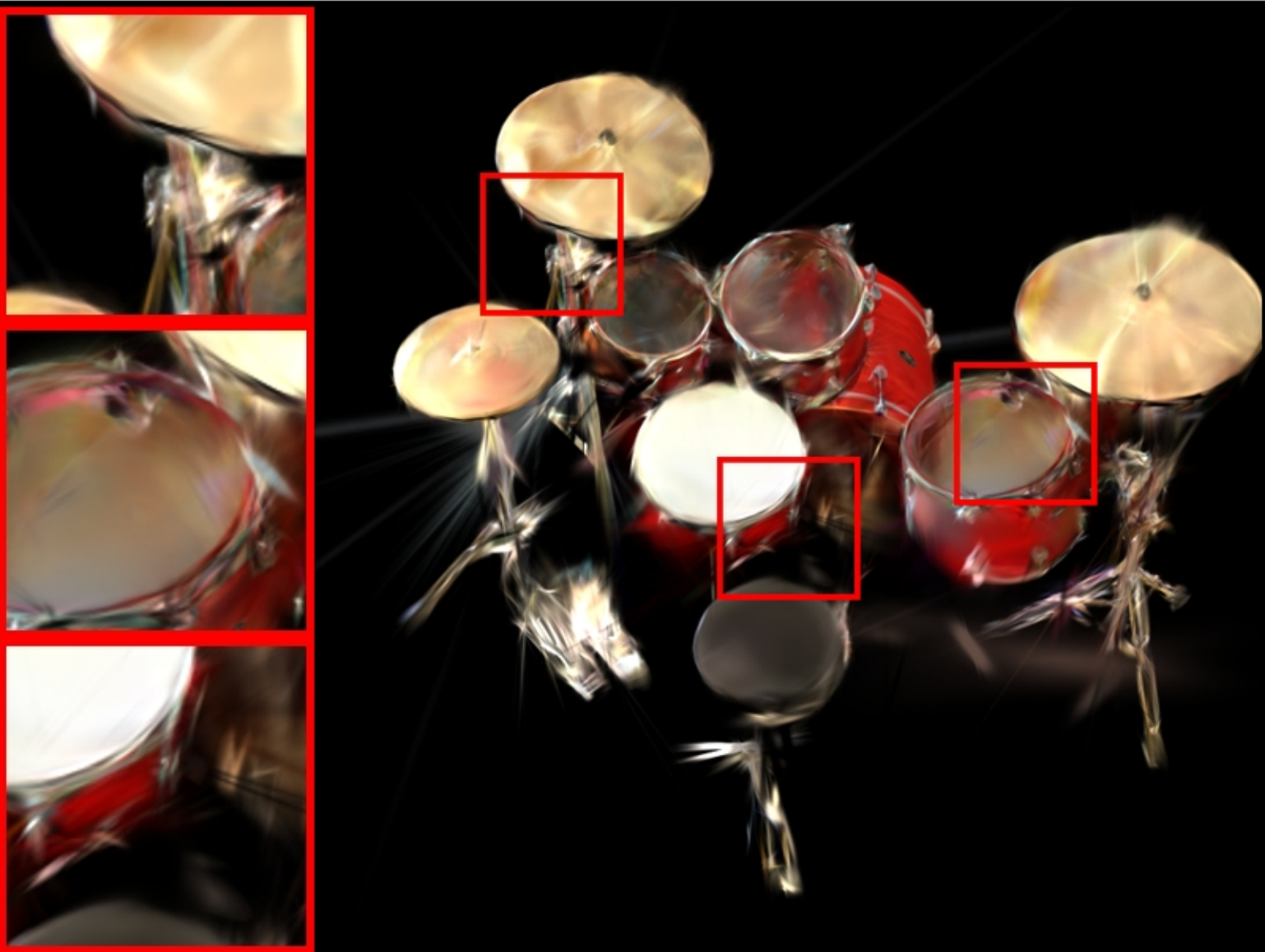
drums: COLMAP | num_images=40 PSNR: 14.85 | LPIPS: 0.2966 | SSIM: 0.6821
