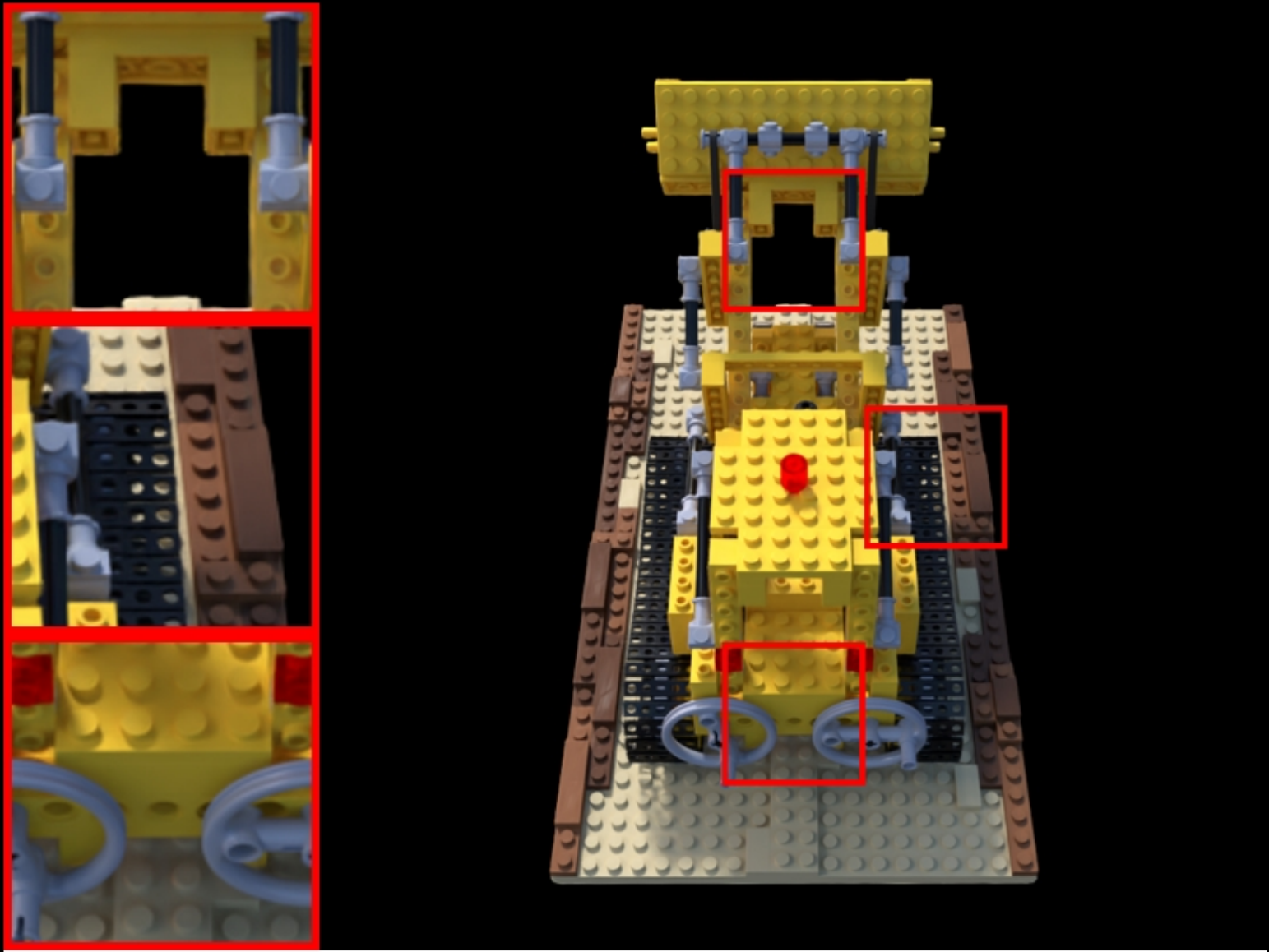
lego: COLMAP | num_images=87 PSNR: 23.94 | LPIPS: 0.0606 | SSIM: 0.8759
