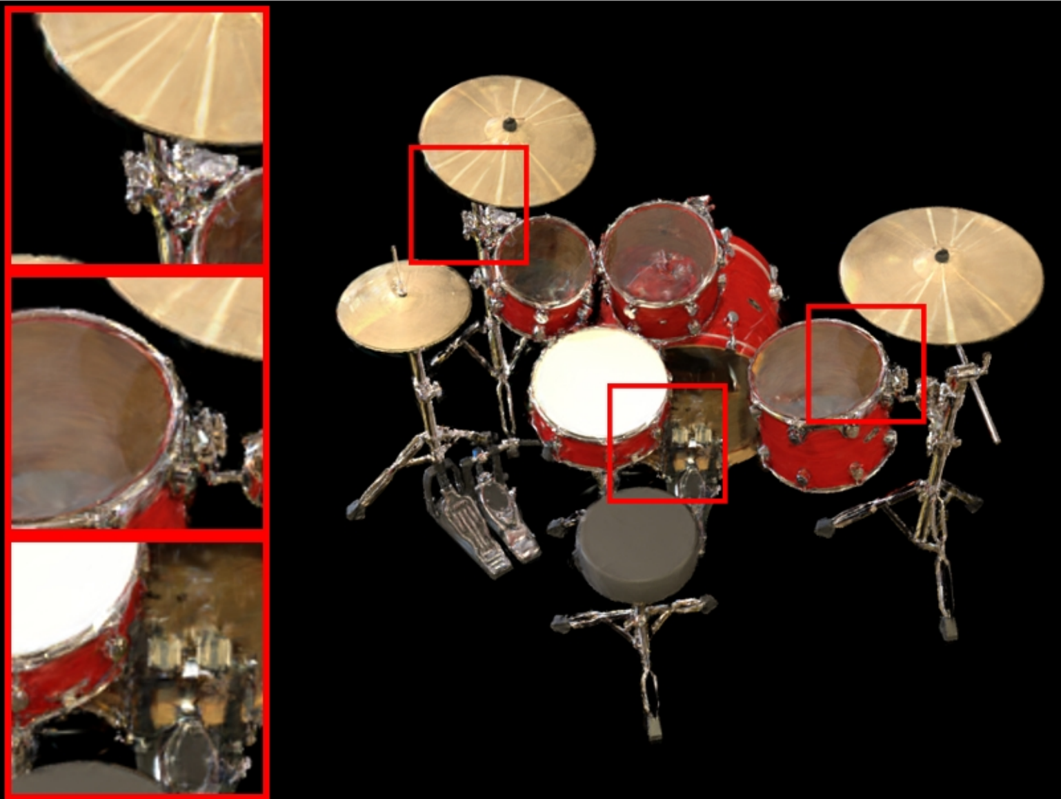
drums: VGGT | num_images=20 PSNR: 18.79 | LPIPS: 0.1023 | SSIM: 0.8142
