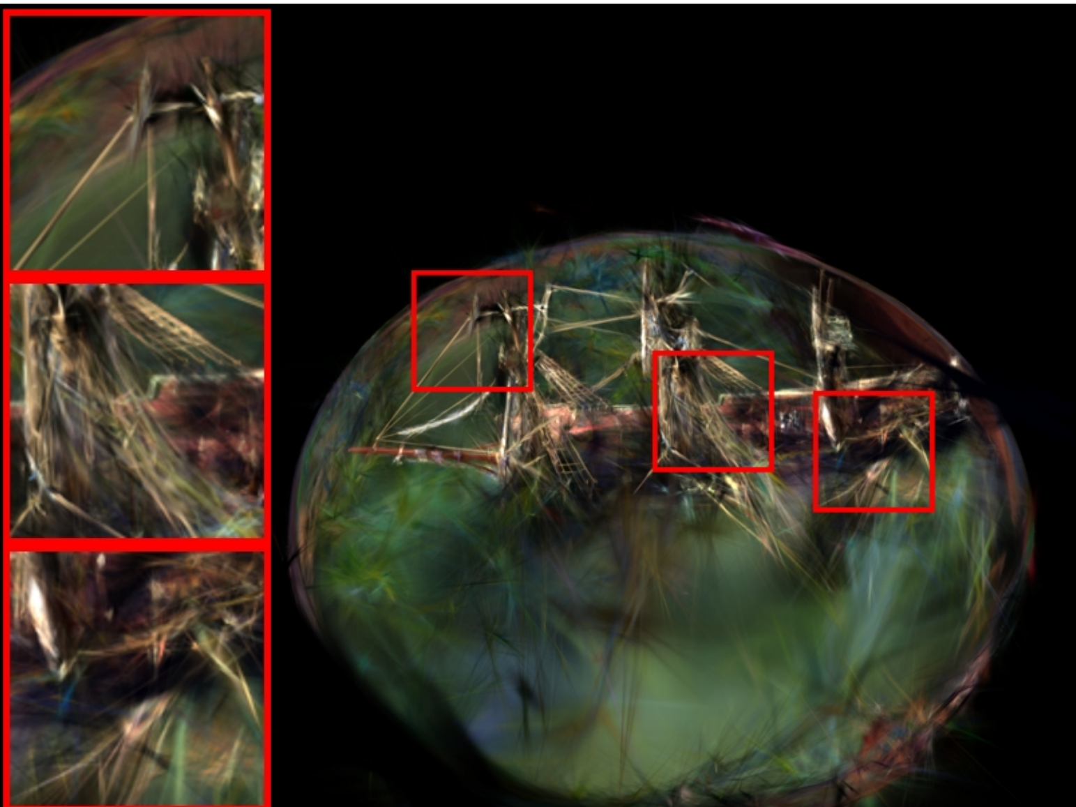
ship: COLMAP | num_images=40 PSNR: 17.97 | LPIPS: 0.3304 | SSIM: 0.6273
