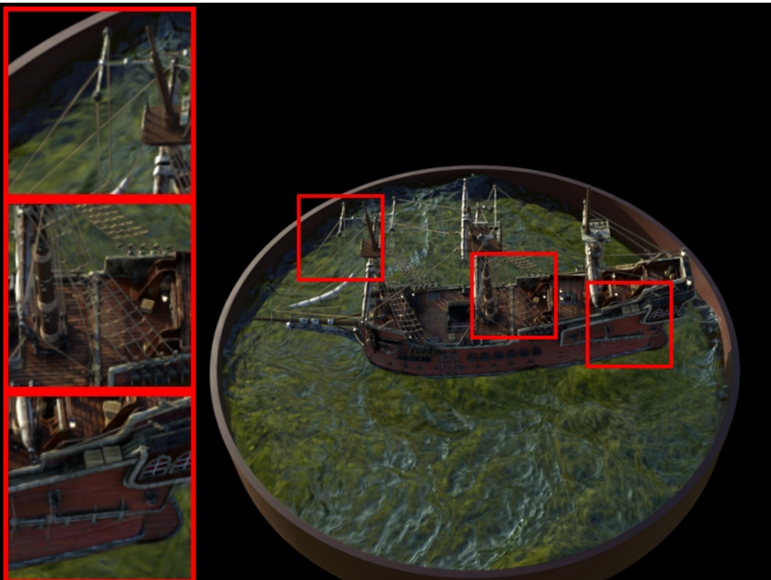
ship: COLMAP | num_images=87 PSNR: 22.54 | LPIPS: 0.1451 | SSIM: 0.7553
