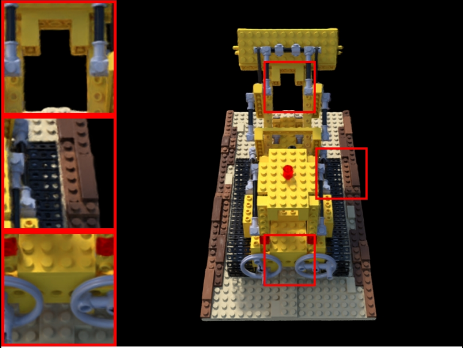
lego: VGGT | num_images=87 PSNR: 20.57 | LPIPS: 0.0950 | SSIM: 0.7736
