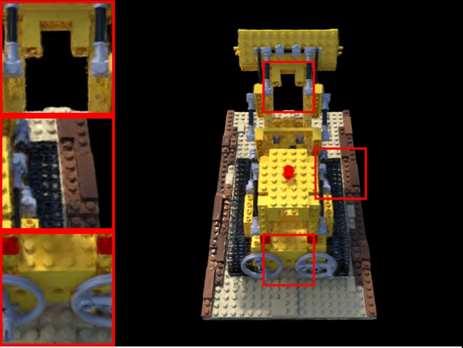
lego: VGGT | num_images=40 PSNR: 21.03 | LPIPS: 0.0892 | SSIM: 0.7866
