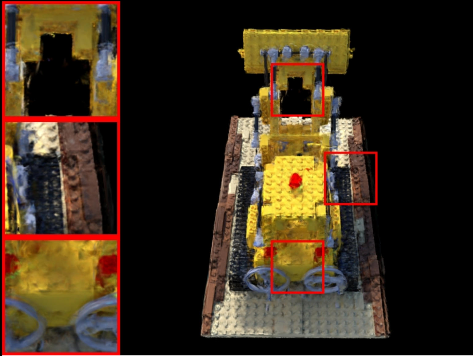
lego: VGGT | num_images=20 PSNR: 17.20 | LPIPS: 0.1505 | SSIM: 0.7221
