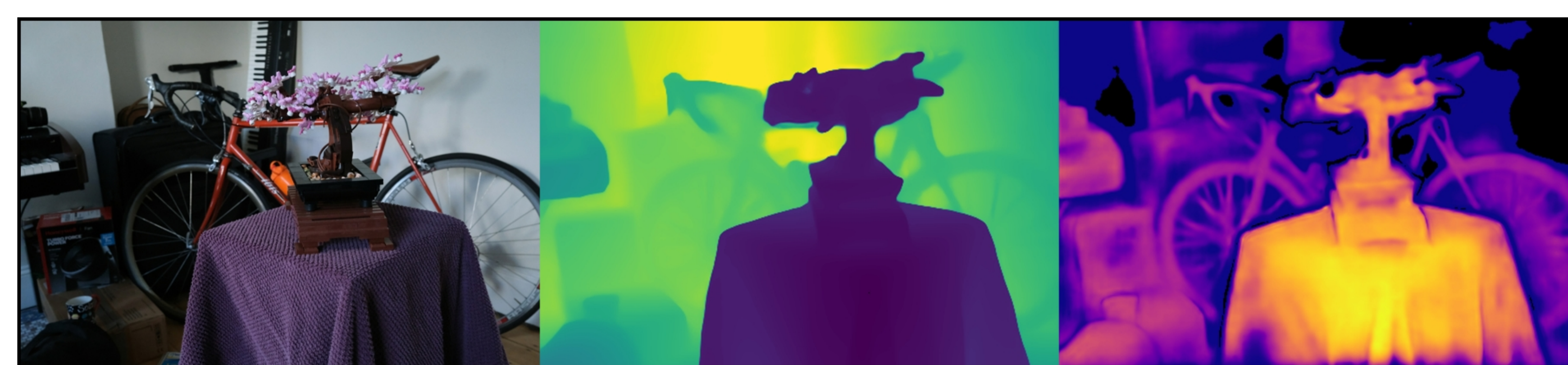
bonsai: VGGT | ba | num_points=23220 Original | Depth (max=2.21) | Confidence (max=5.14)
