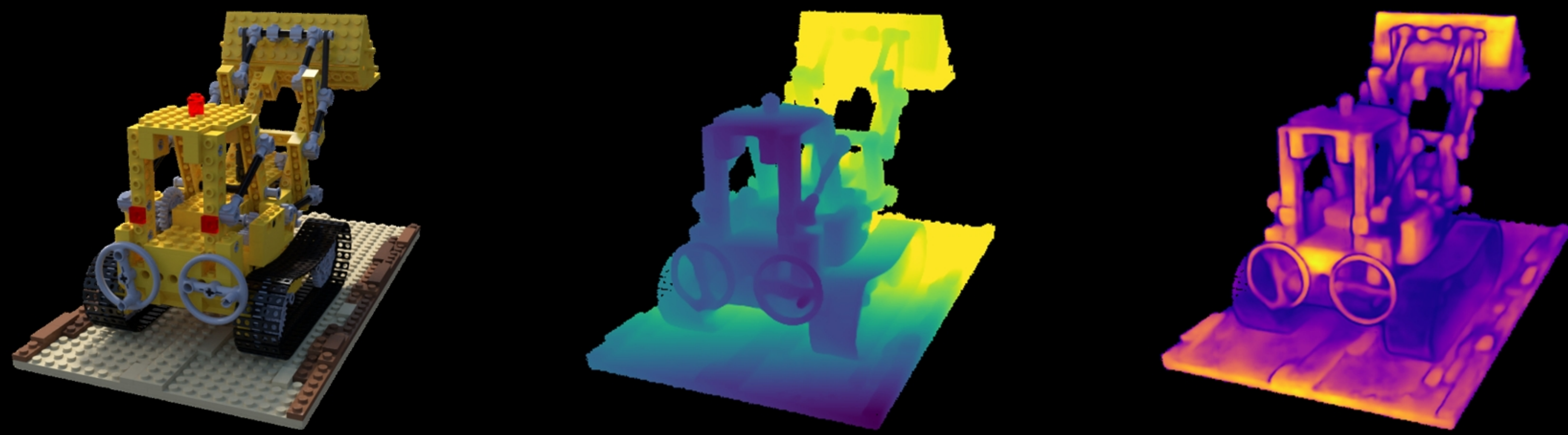
lego: VGGT | confidence | num_points=87000 Original | Depth (max=1.28) | Confidence (max=155.74)
