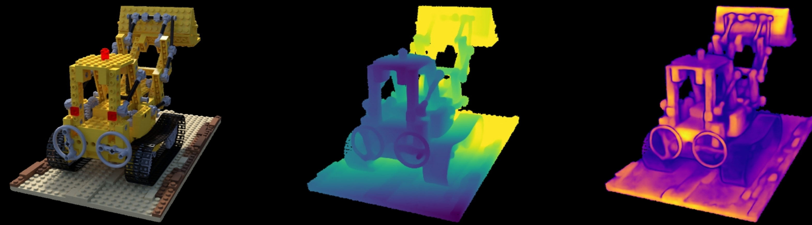
lego: VGGT | imagefps | num_points=87000 Original | Depth (max=1.28) | Confidence (max=155.74)
